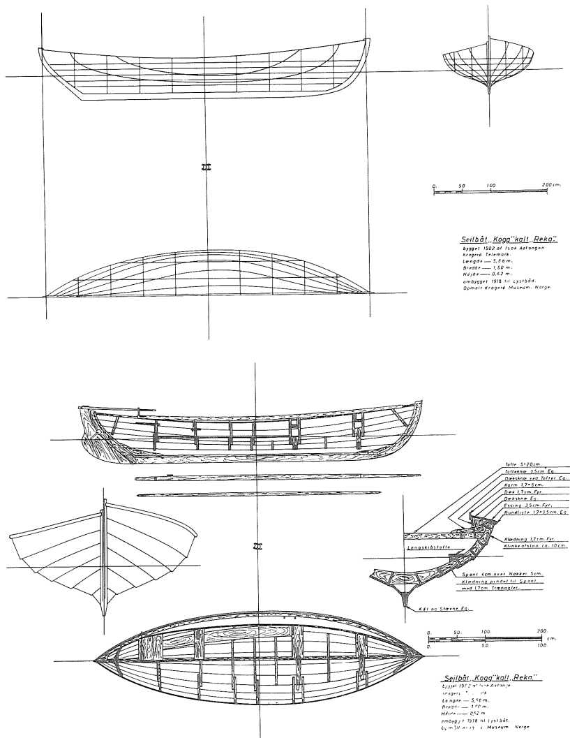
B-kogg »Reka« i Christian Nielsens oppmåling. Drawing of the Reka, a B class cog, done by Christian Nielsen, 1966. Built as a working boat about 1900 and adapted for racing about 1920 the Reka scored many triumphs in regattas with the well known cog sailor Harald Postmyr at the helm.
