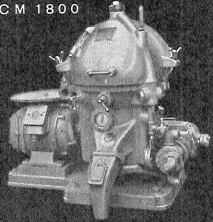
TITAN STANDARD OLIE SEPARATOR TYPE CM 1800
