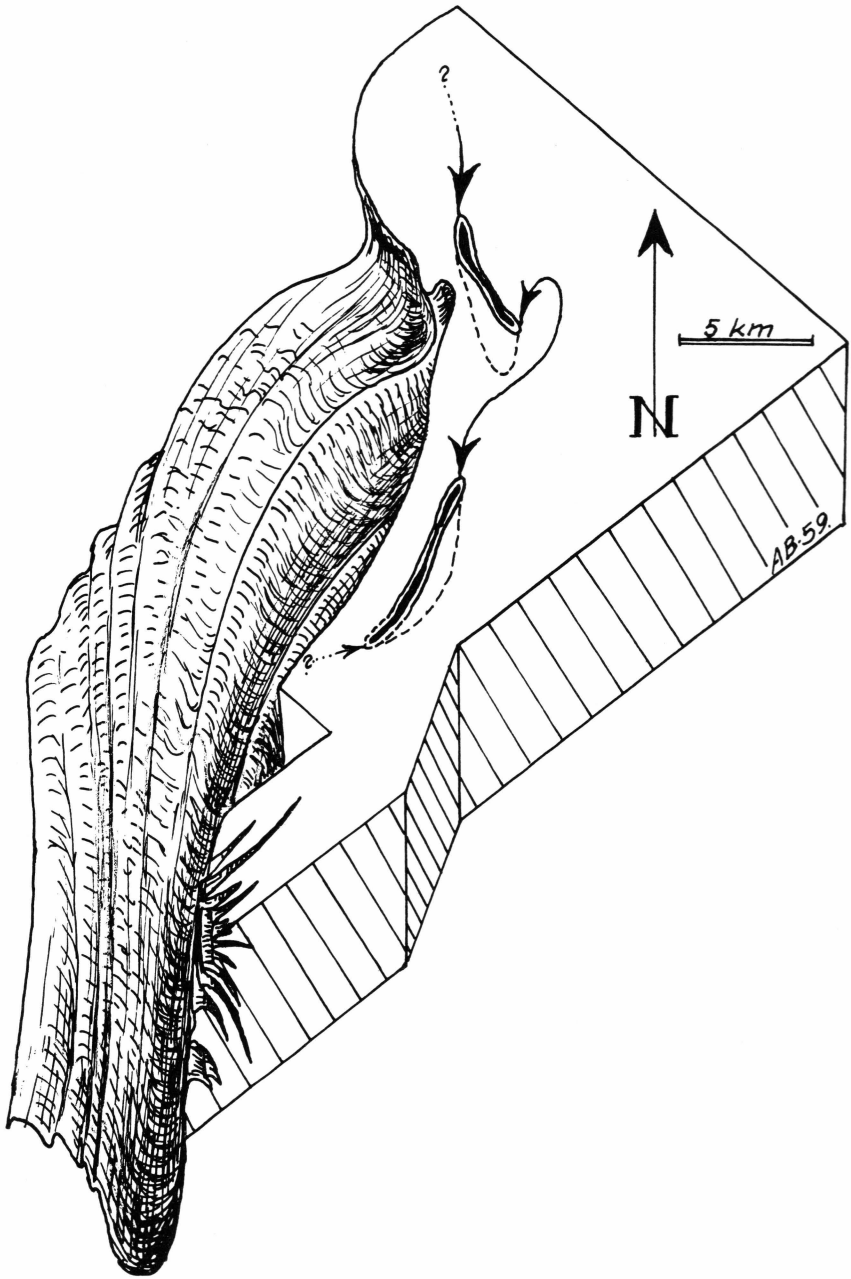
Fig. 16. Tectonogram showing the structural relation between the Alángua complex and the Finnefjeld complex. The depressions and culminations shown by the isoclinally folded amphibolite south of the complex border are also indicated.
