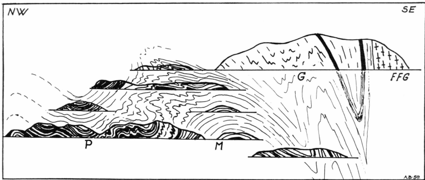
Fig. 14. Composite profile illustrating the fold structures on the islands Igdlutsiait and Portussoq. P: pegmatites, M: migmatitic schists and gneisses, G: gneiss, FFG: Finnefjeld gneiss.
