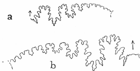
Text-fig. 5. Hectoroceras kochi , sp. nov. Suture-lines of holotype (a), natural size and of specimen figured in Plate II, fig. 1 (b), enlarged \times 2 . (Locs. 313 and 306).
