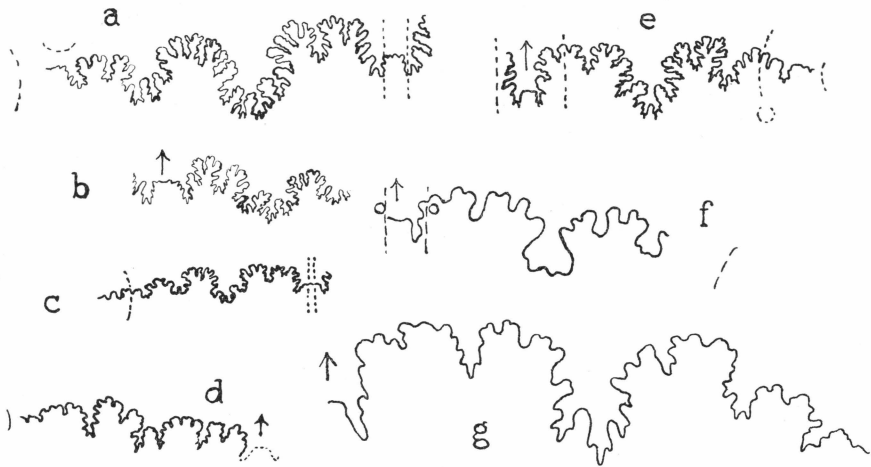
Text-fig. 4. Suture-lines of Pseudogarnieria (a-d), Proleopoldia (e), Delphinites (f), and Neocomites (g). (a). Pseudogarnieria sp. nov. ( Oxynticeras marcoui , Stchirowsky, non d'Orbigny, 1894, pl. xv, fig. 4c). (b). P. undulato-plicatile , Stchirowsky sp. ( ibid. , fig. 3c). (c). P. sp. nov.? ( Oxynticeras gevrili , Stchirowsky sp. ( ibid. , fig. 1c). (d) P. tuberculiferum , Stchirowsky sp. ( ibid. , fig. 2a, from specimen, with external lobe doubtful). (e). Proleopoldia kurmyschensis , Stchirowsky sp. ( ibid. , pl. xvi, fig. 2c). Lower Cretaceous, Alaty, Simbirsk, Russia. (f). Delphinites ritteri , Sayn (1901, fig. 14, p. 23, enlarged \times 4.5 ). (g). Neocomites ("Leopoldia") aenigmaticus , Sayn sp. (1907, fig. 24, p. 55, enlarged \times 5 , reversed for comparison with f). Valanginian, S. E. France.
