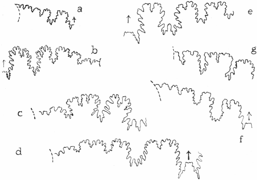
Text-fig. 6. Suture-lines of Subcraspedites . (a). S. stenomphalus , Pavlow sp. (After Pavlow, 1889, pl. III, fig. 10c, Simbirsk, Cent. Russia. (b). S. undulatus , Swinnerton (1935, pl. II, fig. 3B, completed from other, uncrushed side. Spilsby Sandstone, B. M. No. 36352). (c, d). S. primitivus , Swinnerton (at diameters of about 85 and 115 mm. Same bed, Bros. Wright Coll.). (e). S. lamplughi , Spath ( Craspedites subditus , Pavlow, 1892, pl. XIII, fig. 5, B. M. No. C. 34981, Spilsby Sandstone, composite and enlarged about \times 2 ). (f). S. sp. nov. (between S. primitivus , Swinnerton and S. lamplughi , Spath. Spilsby Sandstone, B. M. No. C. 996a. Enlarged \times 1\frac{1}{2} ). (g). S. (?) mutabilis , Stanton (1895, pl. xv, fig. 2). Knoxville Beds, California (enlarged portion of suture-line).
