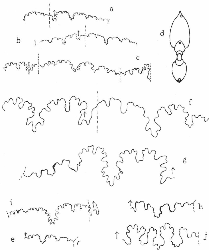
Text-fig. 3. Suture-lines of Platylenticeras (a-h), Tolypeceras (i), and Paquiericeras (j). (a). Platylenticeras heteropleurum (Neumayr & Uhlig). Slightly enlarged, at diameter = 45 mm (B. M. No. C. 13351). (b). P. latum , v. Koenen (1902, pl. I, figs. 1—2). (c-e). P. heteropleurum (Neumayr & Uhlig). Enlarged suture-line at diameter = 35 mm (c) and at 18 mm (e), with cross-section at diameter = 19 mm, enlarged \times 2 (B. M. No. C. 13346). All from Lower Valanginian of Gronau, Westphalia. (f). P. occidentalis , Sayn sp. (1901, fig. 8 on p. 17, enlarged \times 4.5 ). (g). P. cardioceroides , Sayn sp. (1901, fig. 11 on p. 20, enlarged \times 4.5 ). (h). P. nicolasi , Sayn sp. (1901, fig. 12 on p. 22, enlarged \times 4.5 ). Valanginian of S. E. France. (i). Tolypeceras (“ Platylenticeras ”) cuneiforme , v. Koenen sp. (1902, pl. xvi, figs. 4—5). Lower Valanginian, Gronau, Westphalia. (j). Paquiericeras paradoxum , Sayn (1901, fig. 15, p. 26, enlarged \times 4.5 ), for comparison with h. Valanginian, S. E. France.
