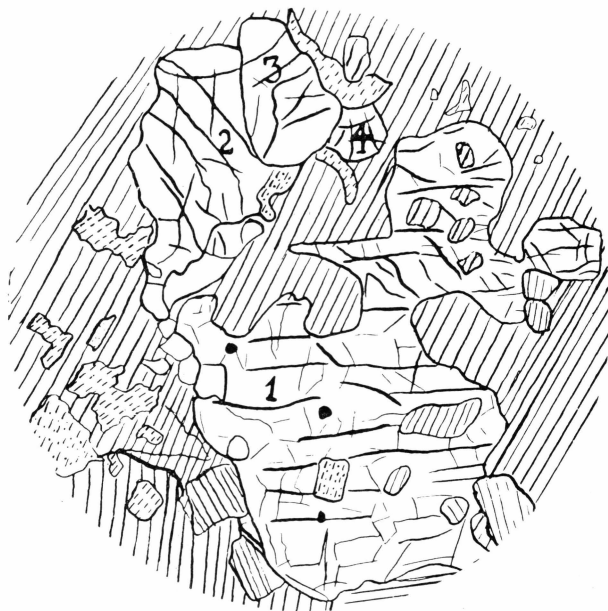
Fig. 8. No. 13449, 16\times , +nic. Corroded grain of olivine (1) surrounded by a large grain of bronzite. "Inclusions" of bronzite in the olivine belong to the same large grain, thus this grain is also found under (or above) the olivine. (Olivine: irregular fractures, bronzite: full lines, diopside: broken lines, hornblende: broken lines and dots, phlogopite: dots). Three small black spots of ore. Bottom left a grain of diopside being replaced by the bronzite. 2, 3 and 4 are small grains of olivine.
