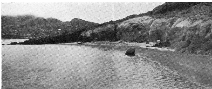
Fig. 4. The dunite to the west of the dyke which is seen behind the boat. A few of the joints in the dunite may be seen. The beach consists of olivine sand.
