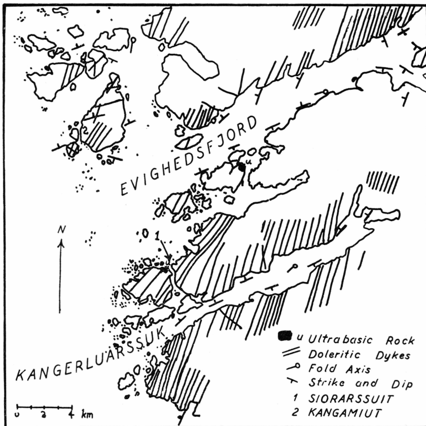
Fig. 1. Geological map of the country around Siorarssuit. The mapping undertaken so far is of a preliminary character, therefore observations are scarce in some areas which explains the casual omission of the dykes of dolerite.
