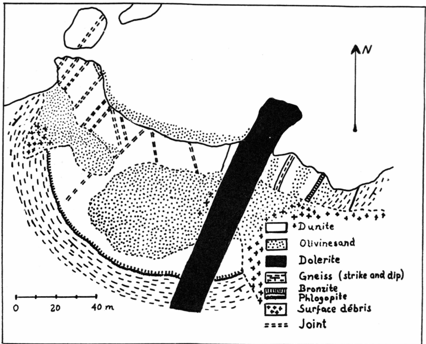
Fig. 2. Geological sketch map of the dunite at Siorarssuit. The map is based on a free hand drawing.
