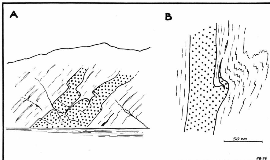
Fig. 2. Metabasaltic dykes. A: partly boudinée, bifurcated metabasaltic dyke. Small headland north of the entrance to the Ameralik-fjord (drawn from a photograph). B: Metabasaltic dyke exhibiting a relic apophysis, which has been folded together with the present flaser-gneiss. South coast of the outer Ameralik-fjord, south of Simiutâ (drawn from a note book sketch).
