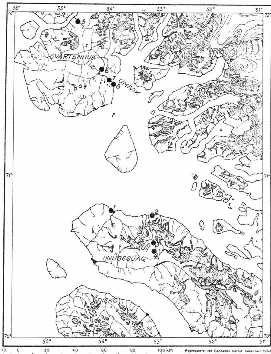
Fig. 1. Map showing the position of localities, where belemnites have been found. Loc. 1: Tuperssuartâ; loc. 2: Ikorfat; loc. 3—4: Angmârtussut; loc. 5: Simiûtap kûa; loc. 6: Firefjeld; loc. 7: Tange IV kløft; loc. 8: Store Tange V kløft.
