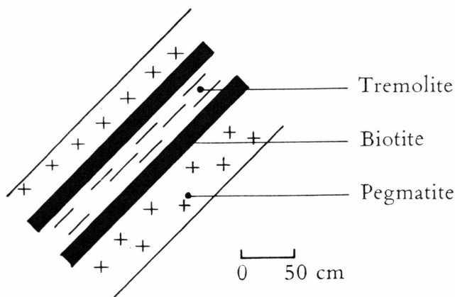
Fig. 25. Tremolite grading into biotite towards the contact with two parallel branches of a pegmatite vein. SW coast of Eqaqut.
