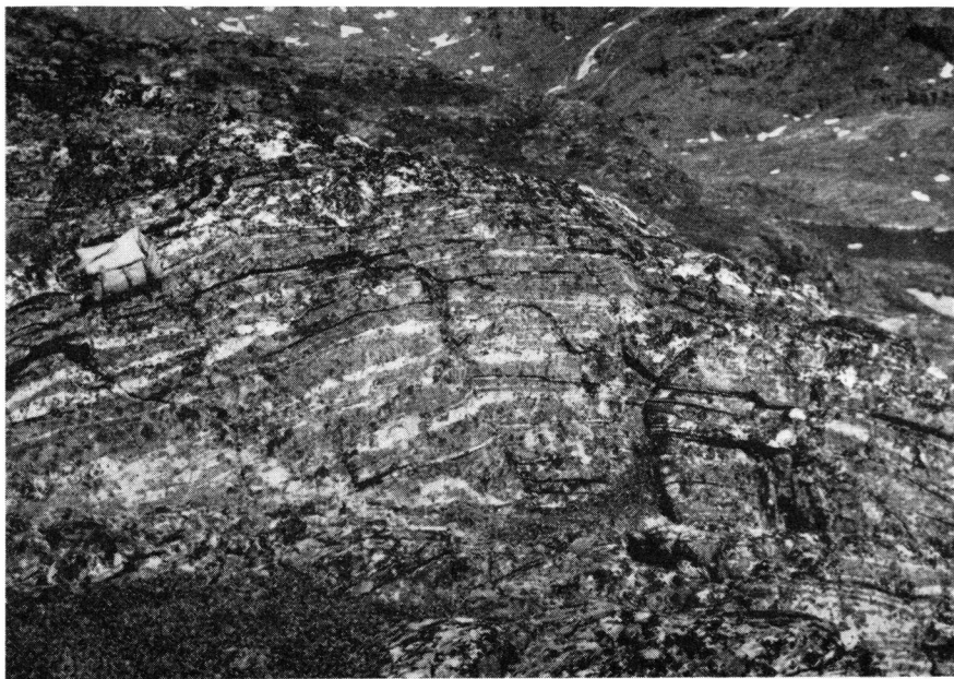
Fig. 29. A gentle, open "charnière" in the vast, southern dome. The rock is banded amphibolitic gneiss. Akuliarusiarssuk.
