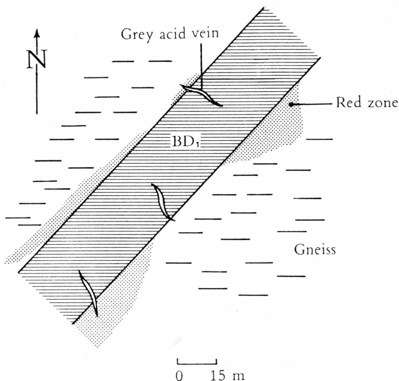
Fig. 58. White or grey acid veins may cut the BD1 perpendicularly, while red zones continue to appear sporadically in the encasing gneiss. As it shall be stated further on, the remobilized gneiss probably back-veins the dolerite. 1 km N of lake 470.
