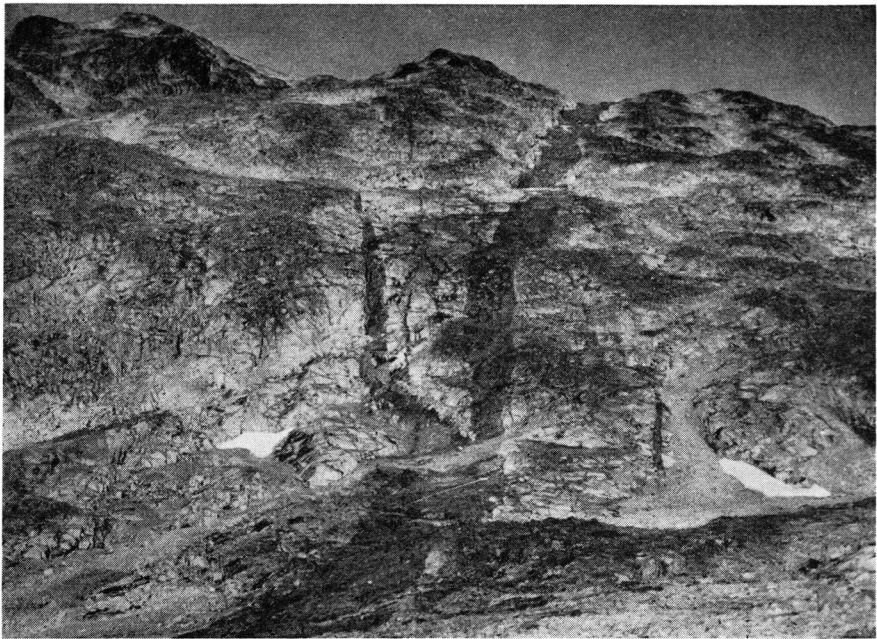
Fig. 47. “En échelon” disposition in a BD. This is a current feature. Sometimes 3, 4 or 5 relays constitute the system. 2 km NW of lake 470.
