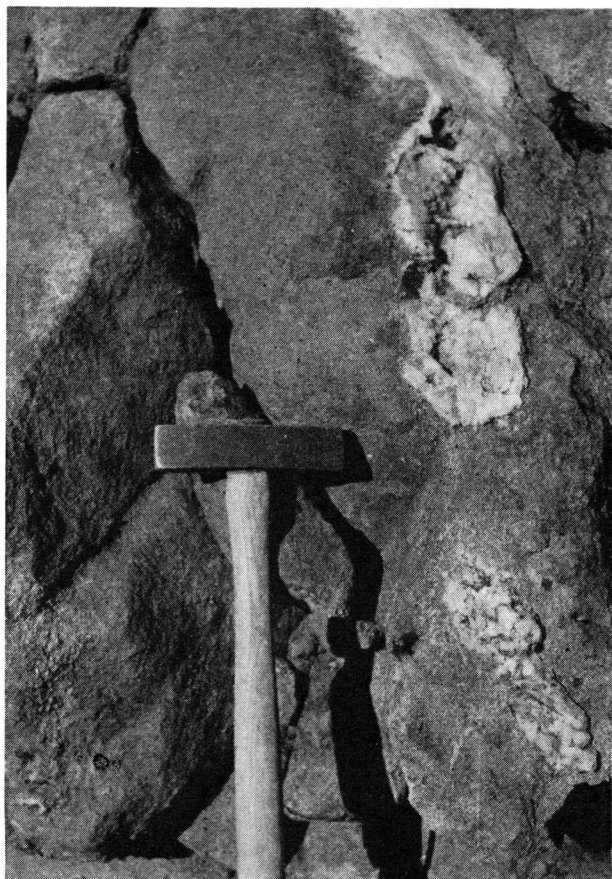
Fig. 52. An acid pegmatite or "pegmatitoide" in a BD1. Patches, spots, streaks or veins of crystallized residual matter may occur. In the case of these dolerites, they are usually of a tonalitic composition. 1 km NE of pt. 812.
