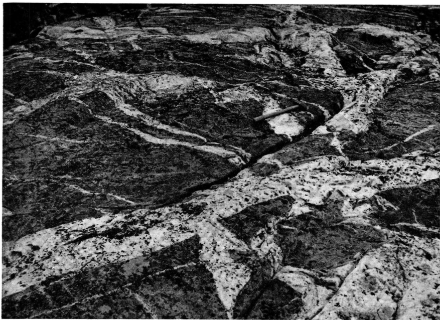
Fig. 19. Network of pegmatites and aplites belonging to several generations, in the agmatitic zones. S coast of Sermiligârssuk.
