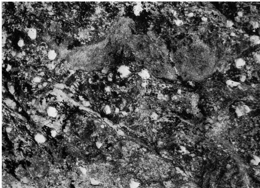
Fig. 34. Big porphyroblasts of plagioclase (about 2-3 cm in diameter) grow in the greenschists of the suprastructure. This is an early stage in the process of migmatization, i.e. feldspathization, which usually precedes, in space as well, the front of the migmatites.
