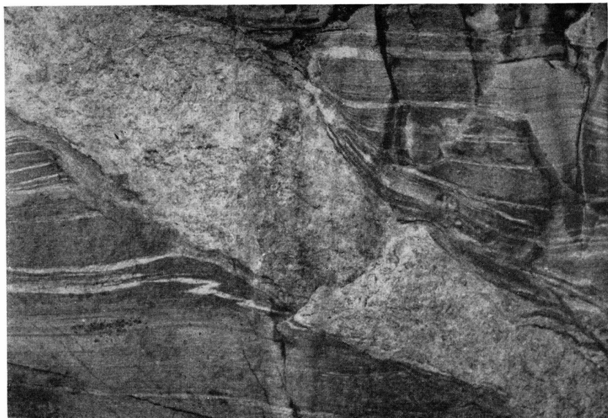
Fig. 18. Bending of the gneissic foliation on either side of a large pegmatite (about 1 m wide). The deformation is probably contemporaneous with the emplacement of the vein. Northern extremity of Kangerdlugssuaq.
