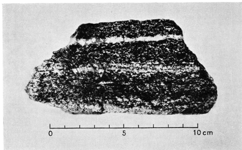
Fig. 8. Banded gneiss, containing essentially oligoclase, quartz, amphibole, epidote and biotite. (No. 32998). Angmassivit.
