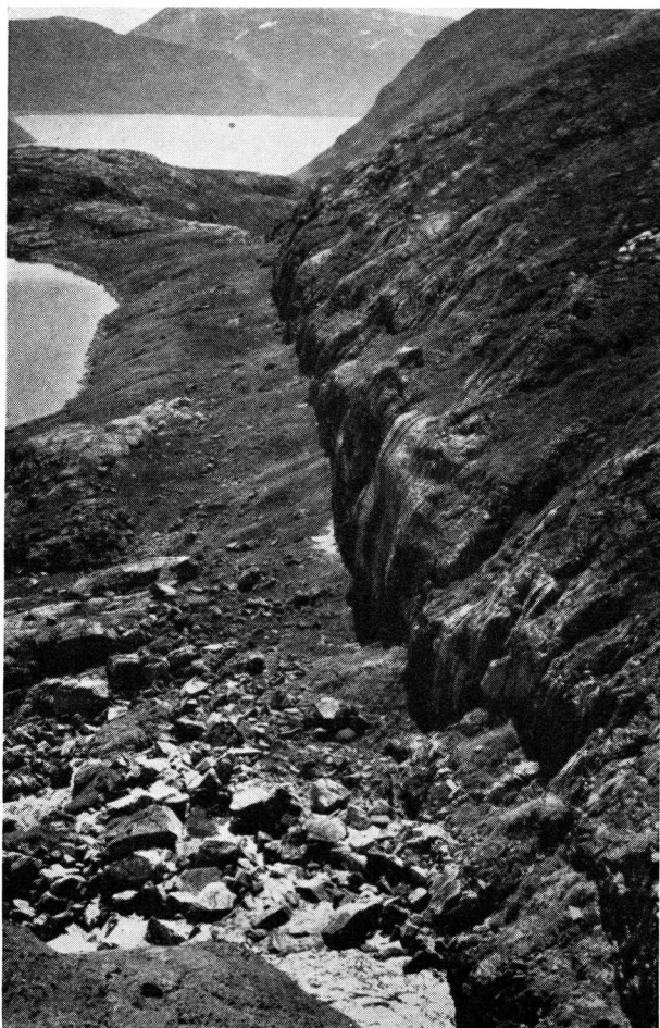
Fig. 59. The big NNE fault which determines Qerrulik.
