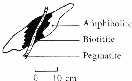
Fig. 23. Replacement, over a few cm, of amphibole by fine flakes of biotite in an amphibolitic lens, due to the emplacement of a small pegmatitic vein.
