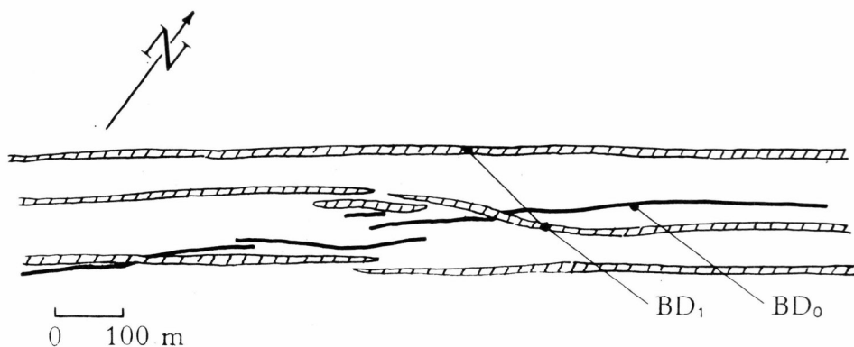
Fig. 54. The swarm of Brown Dykes, where contact phenomena between the dolerites and the encasing gneiss occur. Two generations intersect each other: BD0 and BD1. The effects on the country rock are particularly evident where the easternmost BD1 is "en échelon". 2.5 km NNE of lake 470.
