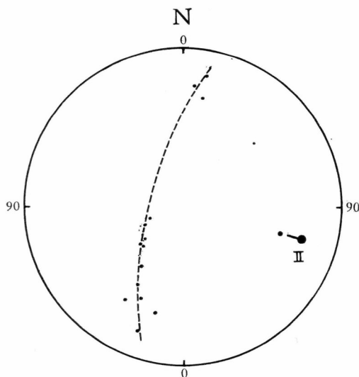
Fig. 32. An example illustrating the use of the Wulf-net. A simple "charnière" in the brachyanticline has been plotted. Dispersion is weak. E of Qerrulik.
