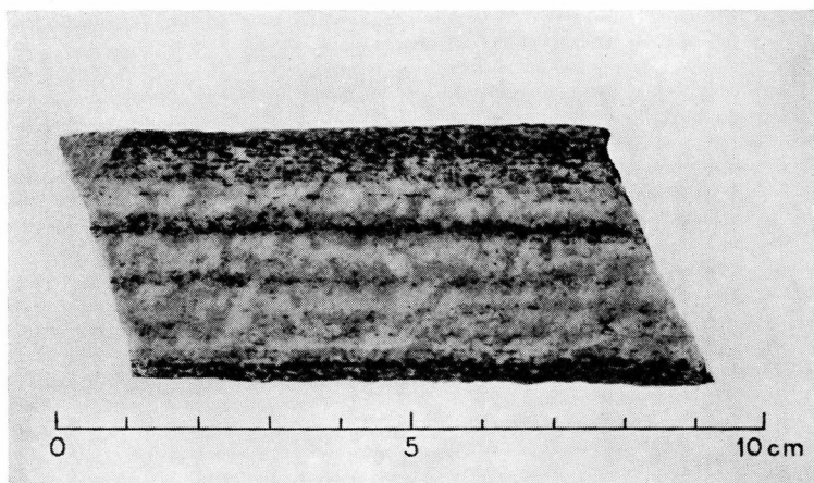
Fig. 9. Banded gneiss, composed of oligoclase, epidote, amphibole, biotite, muscovite and a little microcline, quartz and sphene. (No. 38529). Northern part of Akuliaru-serssuaq.
