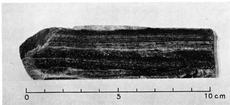
Fig. 5. Slightly migmatized greenschist, containing a great proportion of amphibole, some albite, epidote, and a little quartz, sphene, apatite, calcite, tourmaline and microcline. (No. 38486). Valley of Eqaqut.
