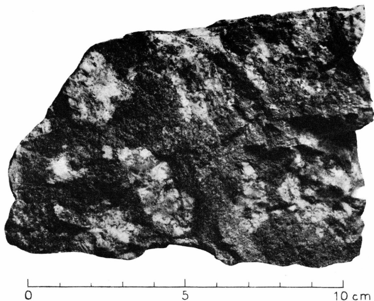
Fig. 50. Xenolithic and phenocrystalline dolerite (BD). The white patches are composed of plagioclase and quartz. (No. 38528). Central part of Akuliaruserssuaq.
