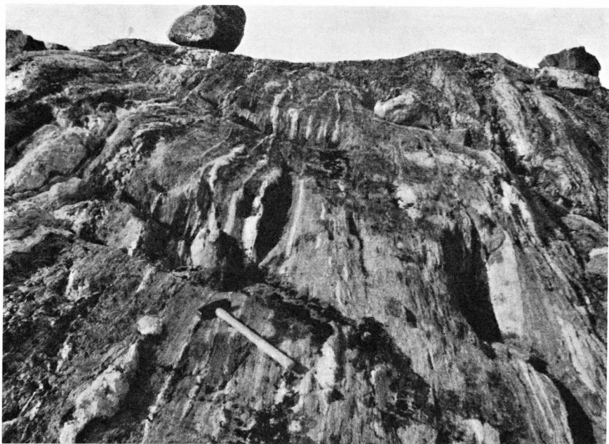
Fig. 3. Detail of the greenschists. Basic and quartzofeldspathic beds alternate quite regularly.
