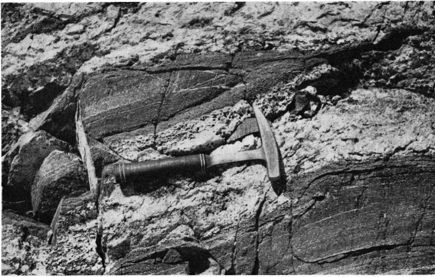
Fig. 37. Hornblendic inclusions surrounded by garnet-rich rims in garnet-biotite augen-gneiss. The big garnets are most clearly visible in the pegmatitized part of the rock, e.g., near the point of the hammer. South of Tigssalûp ilua.
