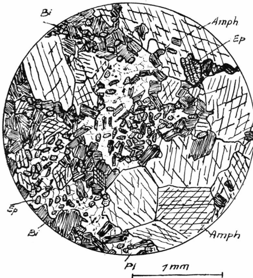
Fig. 27. Epidote-amphibolite, NE. Törnårssuk. Biotite (Bi) has formed at the expense of hornblende (Amph). Epidote (Ep) has developed as interstitial grains in the biotite aggregates. Granular plagioclase (Pl) has replaced much of the biotite and epidote; the latter minerals often figure as inclusions in the plagioclase aggregates. (42035).
