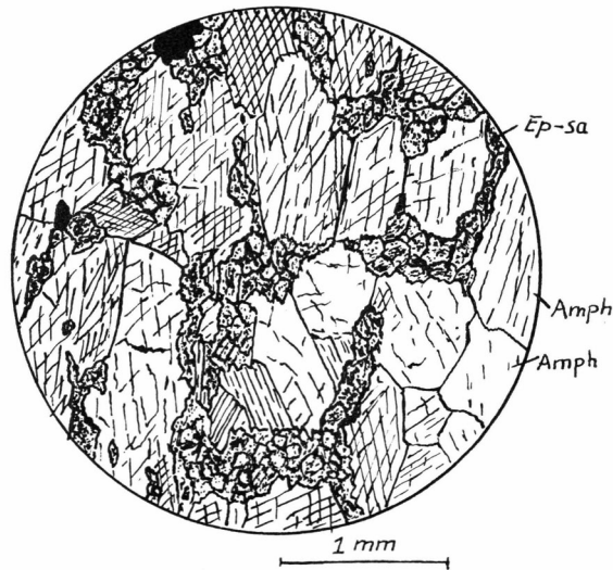
Fig. 20. Epidote-hornblende schist, Kuánit area. Intergranular development of fine-grained saussuritic material and epidote (Ep-sa) at the expense of hornblende (Amph). (46829).
