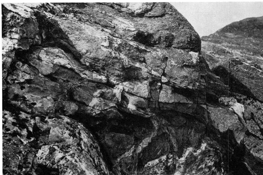
Fig. 6. Biotite-plagioclase-quartz schists thrust upon amphibolites. The schists (upper and left hand part of picture) dip gently to the right and show concordant and subconcordant pegmatitic veinlets. The thicker subconcordant pegmatite with pinch-and-swell structures, and which is shown in the picture running almost diagonally from the upper left hand to the lower right hand corner, has developed partly along the thrust plane (as in the left hand side of picture) and partly just above this plane (as in the central part and lower right hand side of picture). The amphibolites (lower half of picture) dip steeply to the right and contain discordant pegmatitic veinlets, which are bent, broken, and cut off by the thrust plane. Near the thrust plane the amphibolites appear more schistose and they have apparently been subjected to strong shearing. NE. Törnårssuk.
