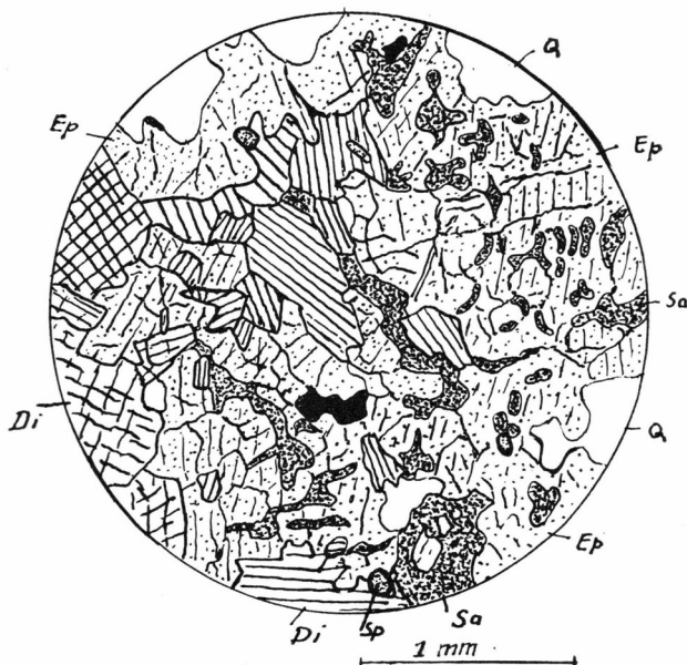
Fig. 22. Diopside-epidote rock, Kuánit area. Epidote (Ep) porphyroblasts have formed by the coalescence of several smaller grains. The saussuritic inclusions (sa) in the epidote separate parts of the porphyroblasts with slightly different extinctions. Diopside (Di) is sometimes found enclosed in the epidote. Other minerals present are quartz (Q) and spene (Sp). (42357).
