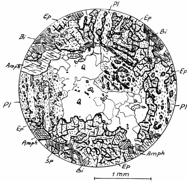
Fig. 29. Quartz-feldspar veinlet in epidote-biotite amphibolite, NE. Törnårssuk. Hornblende (Amph) figures as corroded grains in a mass of biotite (Bi) and epidote (Ep). Plagioclase (Pl) and quartz (Q) form a veinlet in the rock. Corroded epidote inclusions are present in the quartz grains and plagioclase crystals. In the latter mineral the numerous inclusions tend to become arranged parallel to certain crystallographic directions. (42088).
