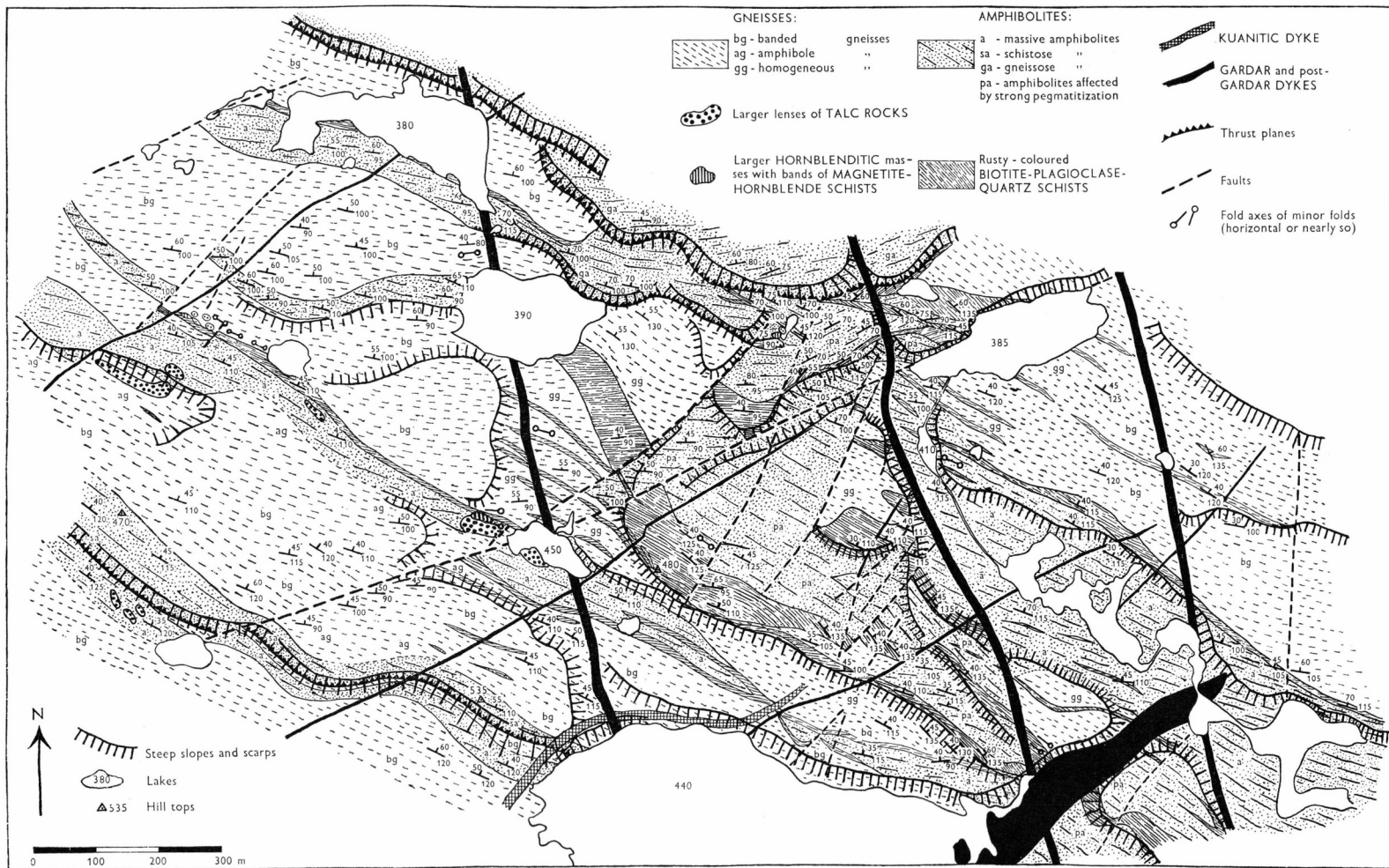
Fig. 3. Geological sketch map of part of NE. Törnärssuk; for location of the area see Fig. 1.
