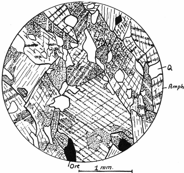
Fig. 26. Magnetite-hornblende schist, NE. Törnärssuk. The amphiboles (Amph) consist of homoaxial intergrowths of alternating lamellae of a colourless, probably tremolitic amphibole and a blue green hornblende, polysynthetically twinned according to (001). The amphiboles are corroded by quartz (Q). Black is magnetite. (42132).
