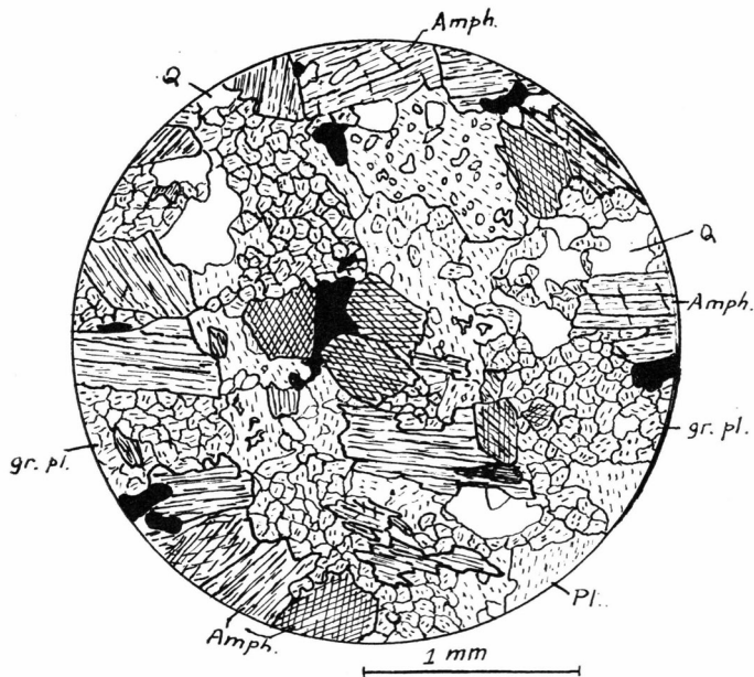
Fig. 23. Amphibolite, Kuánit area. Corroded hornblende (Amph) aggregates figuring in a matrix of granular plagioclase (gr. pl) and quartz (Q). Some plagioclase porphyroblasts (Pl) showing graphic intergrowths with quartz have developed in the granoblastic groundmass. (46858).
