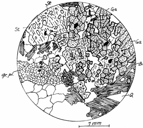
Fig. 32. Staurolite-garnet-biotite augen-gneiss, South of Tigssalûp ilua. Staurolite (St) has penetrated the garnets (Ga) along fractures. Other minerals shown are biotite (Bi), quartz (Q), and granular plagioclase (gr. pl). (42321).
