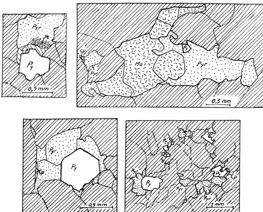
Fig. 16. Ore minerals in the hornblendites and epidote-hornblende schists. Pyrite (Py), pyrrhotite (Pyr), chalcopyrite (Cp), pentlandite (Pe), and magnetite (Ma).
