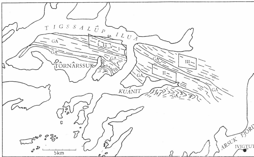
Fig. 1. Sketch map of the gneiss area NW. of Ivigtut with the locations of the investigated areas. I. NE. Törnárssuk, Ia. location of the map of Fig. 4; II. the Kuánit area; III. the area south of Tigssalúp ilua. GA. the "gabbro-anorthosite series". (After a map compiled by A. BERTHELSEN).
