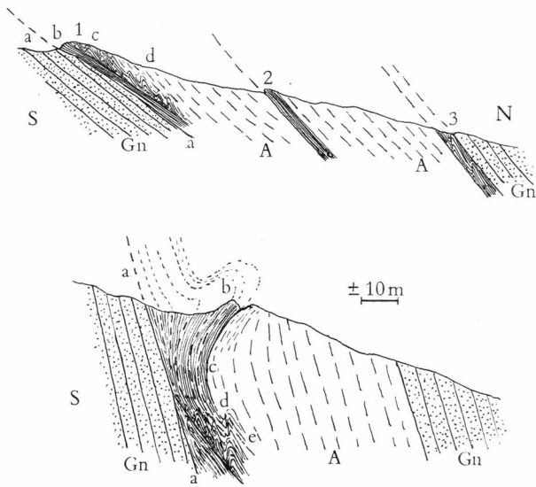
Fig. 14. Generalized diagrammatic representation of some field relations on NE. Törnârssuk and in the area south of Tigssalûp ilua. Upper figure: NE. Törnârssuk. 1. Zone of biotite-plagioclase-quartz schists on the foot wall side of amphibolitic layer; a-a, locally concordant and locally discordant contacts with the underlying gneisses (Gn), at places the contact appears to be a thrust plane (e.g. Fig. 6); b, strongly schistose zone showing microplications, rotated and drawn-out inclusions (Fig. 7), contorted pegmatitic veinlets (Fig. 9) and other signs of shearing movements; c, small-scale folds (Figs. 5 and 8), mostly southerly directed recumbent folds often with hornblendic relics in the hinge zones; d, gradual transitions of biotite-plagioclase-quartz schists into amphibolites (A). 2. Zone of biotite-plagioclase-quartz schists intercalated in amphibolites; the schists often show a slight discordancy with regard to either the underlying or overlying amphibolites. 3. Biotite-plagioclase-quartz schists on the hanging wall side of amphibolitic layer; sharp contacts between amphibolites and biotite-plagioclase-quartz schists.
