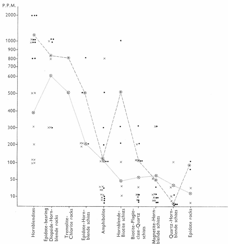
Fig. 33. Results of semi-quantitative spectrographic analyses for Cr and Ni in hornblende rocks and their polymetamorphic derivatives from NE. Tôrnârssuk and the Kuánit area. Dots represent Cr-values; crosses Ni-values; average values are circled. Analyst Mr. IB SØRENSEN.
