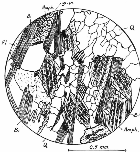
Fig. 25. Biotite-hornblende schist, Kuánit area. The idioblastic amphiboles (Amph) consist of a colourless, probably tremolitic amphibole with lamellae of blue green hornblende in the central parts of the larger crystals; parallel to the lamellae are trains of quartz inclusions. Quartz (Q) forms a granoblastic groundmass. Plagioclase (Pl) is present as porphyroblasts and in fine-granular aggregates. Biotite (Bi) forms relatively large subhedral flakes. (46845).
