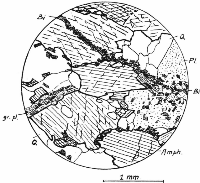
Fig. 28. Amphibolite, NE. Törnårssuk. Interstitial development of biotite (Bi) between the hornblendes (Amph) and along a crack in the rock. Biotite and hornblende are replaced by plagioclase (Pl) and quartz (Q). The biotite veinlet traversing the hornblende crystals is still recognizable in the plagioclase, although in the latter mineral it appears to have been disordered. Granular plagioclase (gr. pl) have locally replaced biotite aggregates. (42115).
