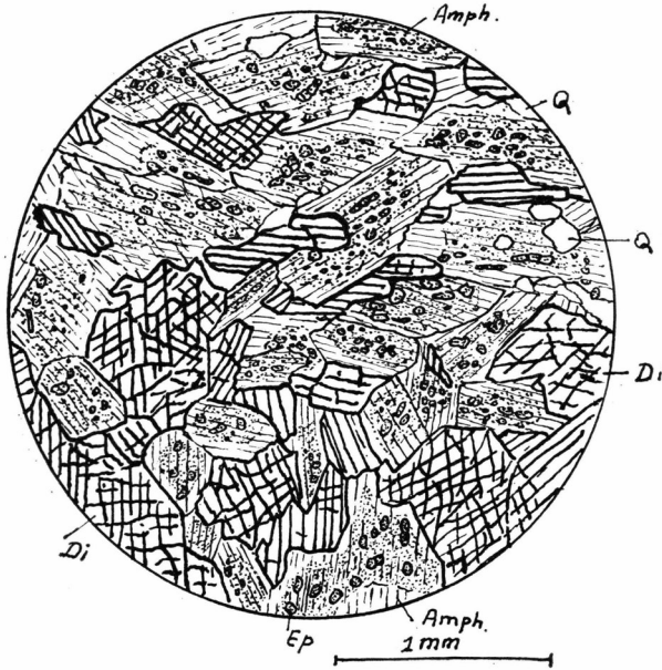
Fig. 17. Hornblende-diopside rock, Kuánit area. The amphiboles (Amph) have a core of bluish green hornblende surrounded by a rim of colourless, tremolitic hornblende. The bluish green core is replaced by epidote (Ep). Diopside (Di) appears quite fresh. Quartz (Q) is sparingly present. (46848).
