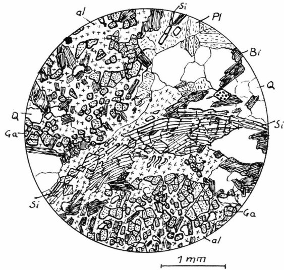
Fig. 31. Garnet-sillimanite-biotite augen-gneiss, South of Tigssalùp ilua. The dense aggregates of sillimanite (Si) contain some relic biotite (Bi) flakes. The sillimanite needles are bent and broken by the garnet (Ga) porphyroblasts. The garnets have been partly replaced by biotite. Late albite (al) occurs as large grains replacing sillimanite, garnet, biotite, andesine (Pl), and quartz (Q). (46884).
