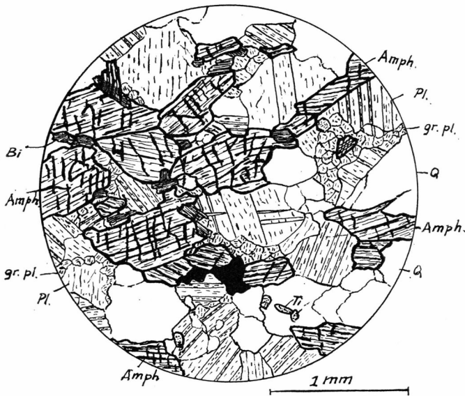
Fig. 24. Amphibolite, Kuánit area. Corroded hornblende (Amph) aggregates figuring in a matrix of coarse-grained plagioclase (Pl) and quartz (Q). Finely granular plagioclase is locally present (gr. pl). Some biotite (Bi) has developed interstitially between the amphiboles. Spene (Ti) is an accessory mineral. (46842).
