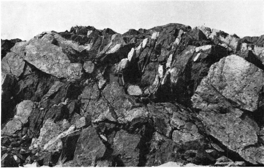
Fig. 8. Small-scale folds along a zone of biotite-plagioclase-quartz schists. The concordant pegmatites are affected by the folding and broken into pieces. The pieces in the limbs of the fold have been affected by shearing and were broken again into a series of smaller pieces. Further shearing will presumably result in the type of small, concordant pegmatites as shown in Fig. 9. NE. Tôrnârssuk.
