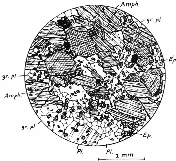
Fig. 21. Epidote-amphibolite, Kuánit area. Epidote granules (Ep) have developed interstitially between the hornblende crystals (Amph). Epidote and hornblende are replaced by granular plagioclase (gr. pl) aggregates, in which plagioclase porphyroblasts (Pl) have developed. (42332).
