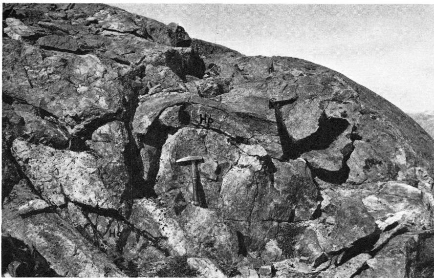
Fig. 11. Hornblende inclusions (Ho) in garnet-biotite augen-gneiss south of Tigssalûp ilua. The inclusions often occur in the hinge zone of folds.
