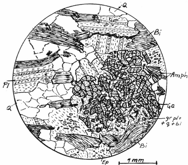
Fig. 30. Garnet-bearing biotite-plagioclase-quartz schist, NE. Törnärssuk. The garnet (Ga) porphyroblasts have deformed the biotite (Bi) flakes. Some relic grains of amphibole (Amph) are enclosed in the garnet. The garnet is partly replaced by a fine-grained aggregate of granular plagioclase (gr. pl), biotite, and quartz. Plagioclase porphyroblast (Pl) sometimes contain inclusions of epidote (Ep) granules. (42250).
