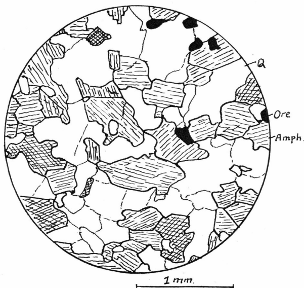
Fig. 19. Quartz-hornblende schist, Kuánit area. The hornblende (Amph) appears as corroded grains and aggregates in a quartz (Q) matrix. (46933).
