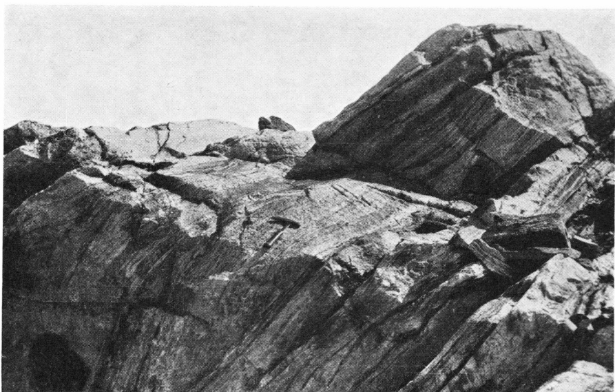
Fig. 4. Sedimentary features in the banded gneisses on NE. Tôrnârssuk (near lake 440).
