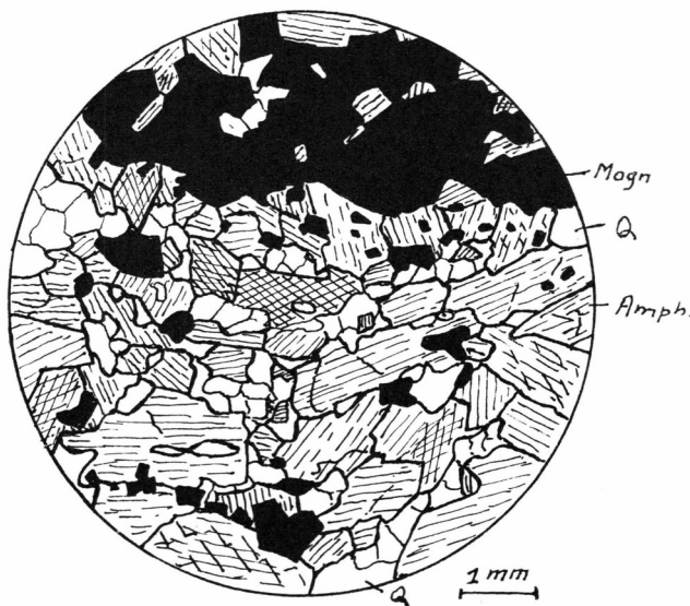
Fig. 18. Alternating bands of magnetite-hornblende schist and quartz-hornblende schist, Kuánit area. Quartz (Q) has developed interstitially between the amphiboles (Amph). Black is magnetite. (42351).
