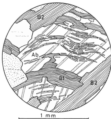
Fig. 8. Aggregates of sillimanite needles (Si) enclosed in late albite (Ab). The sillimanite needles themselves are not bent, but are arranged along a pre-existing curvature in the biotite flake which they partially replaced. Two biotite generations can be seen (B 1 and B 2). Slide No. 51625.
