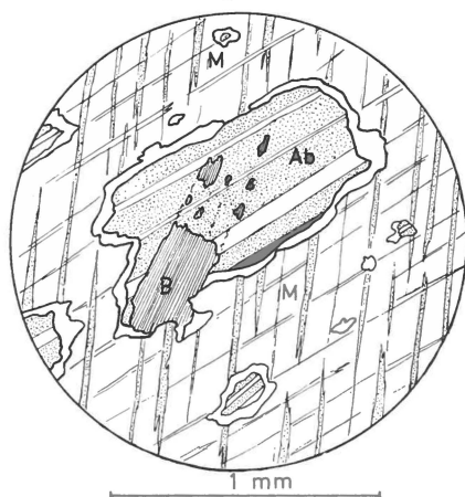
Fig. 36. Inclusion of albite-oligoclase (Ab) and biotite (B) in a large microcline crystal (M). It is evident that the plagioclase partially replaced the biotite, whilst the late microcline grew at the expense of both the plagioclase and biotite. The clear rim around the inclusion is formed by albite. Granite B near Aniggoq mountain. Slide No. 63627.
