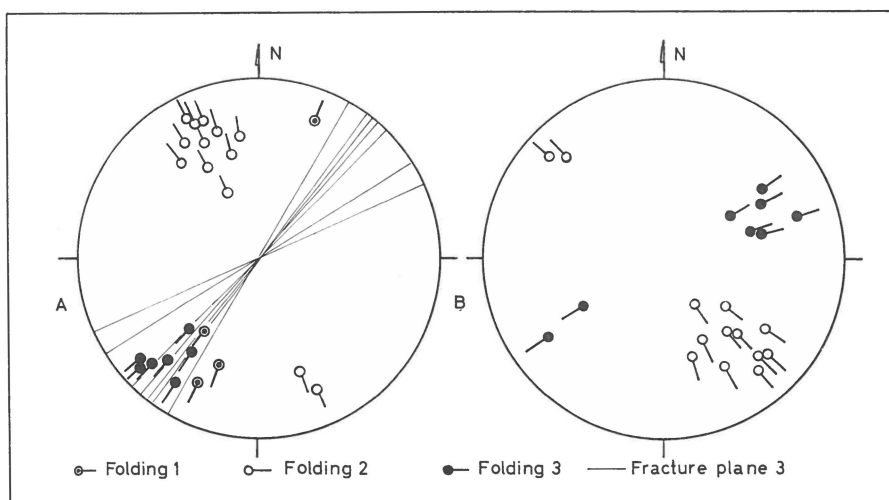
Fig. 7. A: Stereogram of smallfold-axes and orientation of the joints resulting from the fracture-cleavage in the area east of lake 430 m. B: Stereogram of smallfold-axes from the region around Nanortalik (Wulff net, lower hemisphere).
