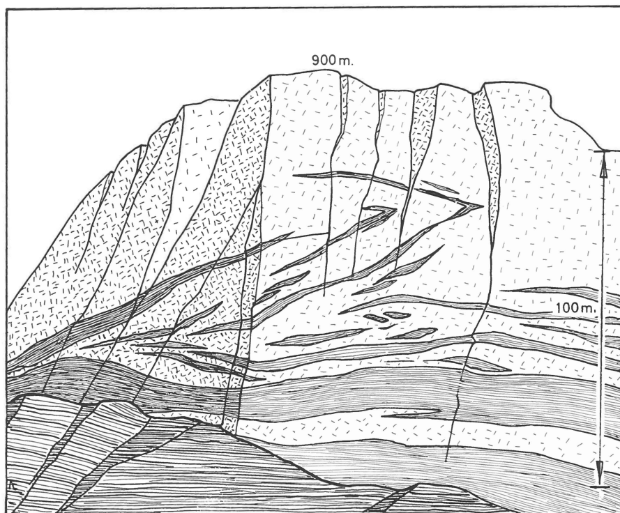
Fig. 24. View of the SW wall of the ridge below the summit of Quvnerssuaq mountain. The granite A, forming the top of the ridge, contains relicts of schists bent in a recumbent fold.
