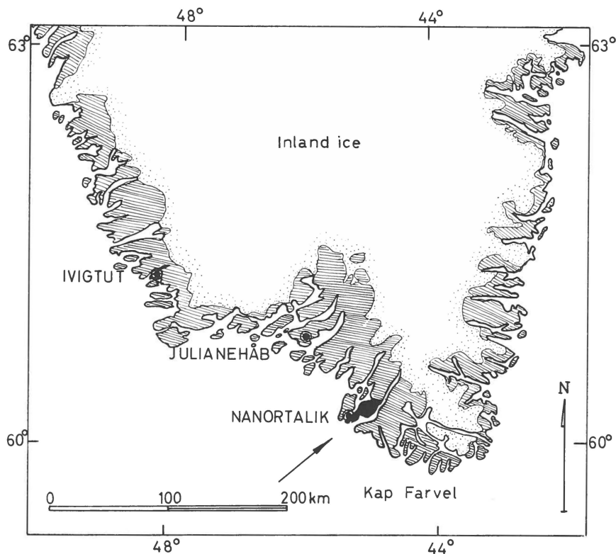
Fig. 1. Map showing the southern part of Greenland and the location of the area under consideration.
