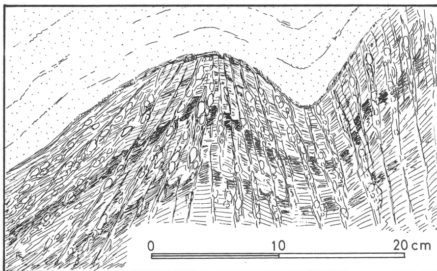
Fig. 20. Feldspar porphyroblasts growing as "augen" in fracture-cleavage planes cutting gneissic schists. Tusardluarnâq peninsula.
