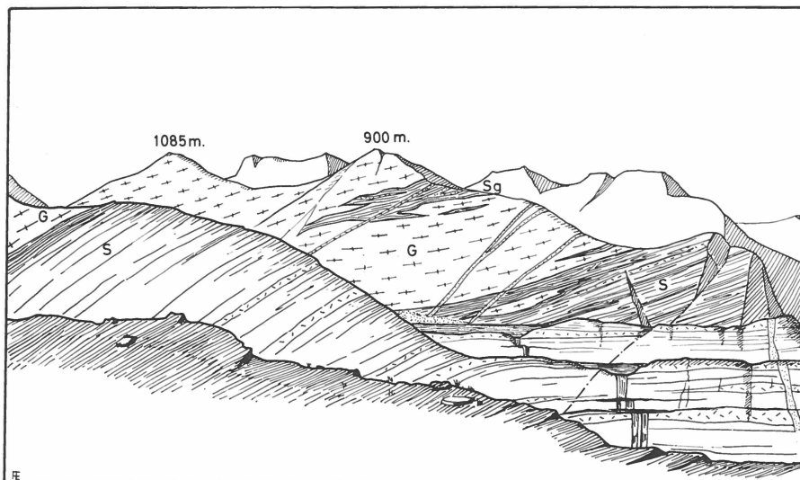
Fig. 25. View from the S of the mountains bordering lake 430 m. Granite A (G) lies conformably upon pelitic schists (S), belonging to the base of unit III. It contains a large undisturbed inclusion of garnet schist (Sg).
