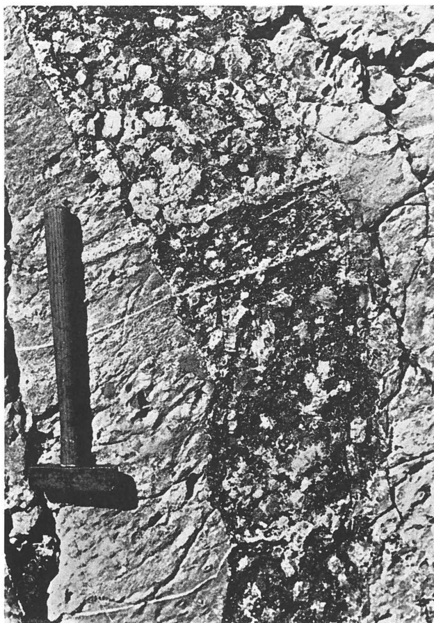
Fig. 38. Discordant vein of granite B in quartzite. Small island in Tasermiut fjord near Aniggoq mountain.
