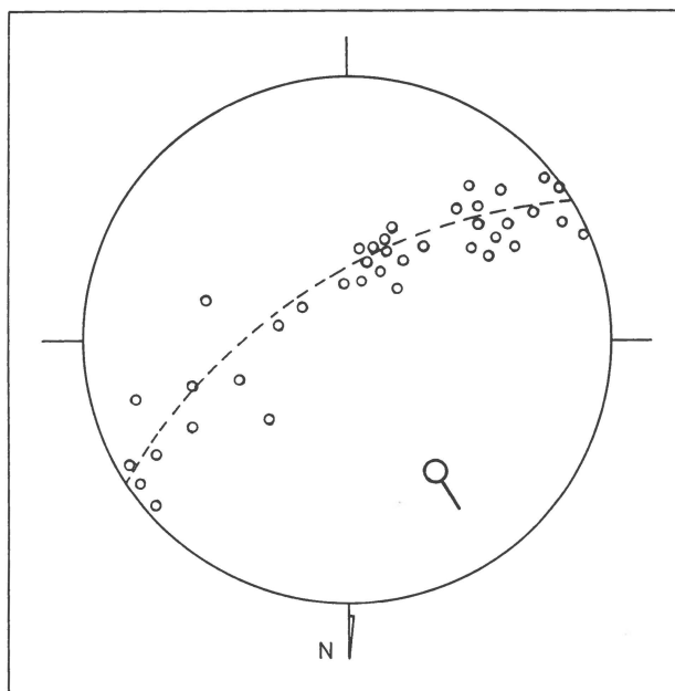
Fig. 27. Stereogram of the foliation poles of 39 large and small inclusions of volcanic rock in granite in the upper part of the synclinal valley between the summits 985 and 875 m (see fig. 26). The lower hemisphere of the Wulff net is used.
