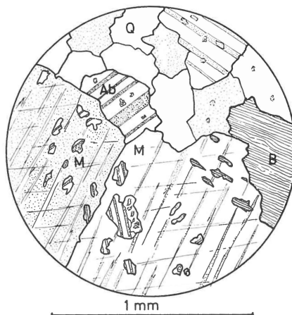
Fig. 43. Microcline (M) partially replacing biotite (B) and albite-oligoclase (Ab) in a vein of granite C. Slide No. 63642.
