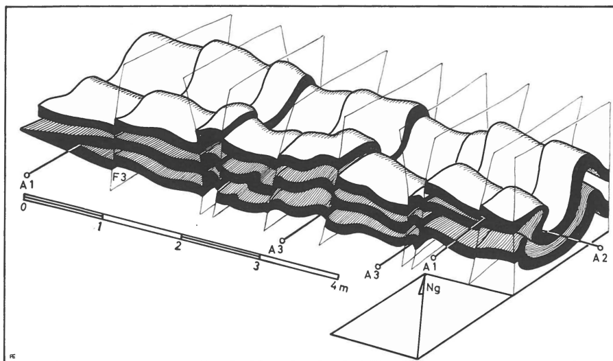
Fig. 6. Simplified reconstruction of a multiple-folded pyritic schist layer in the garnet-mica schist formation near lake 430 m (North of Quvnerssuaq). It is clear that the NW-folding (axis A 2) refolds the earlier formed isoclinal fold (axis A 1), while the coarse strain-slip-cleavage (F 3) cuts the whole structure.
