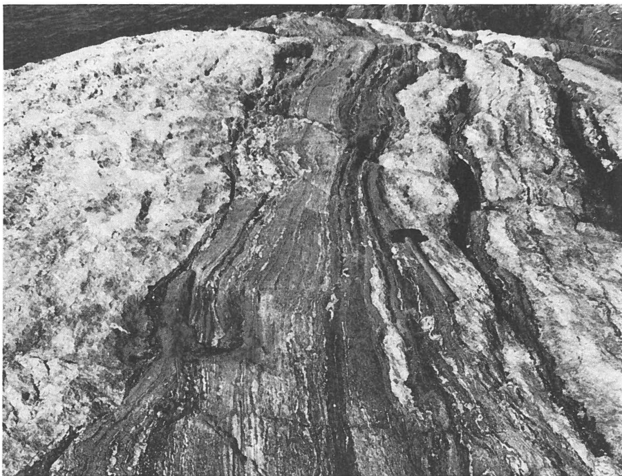
Fig. 14. Fourth-generation, large pegmatites concordant with the foliation. Gneissic schist formation on a small island S of Nanortalik harbour.
