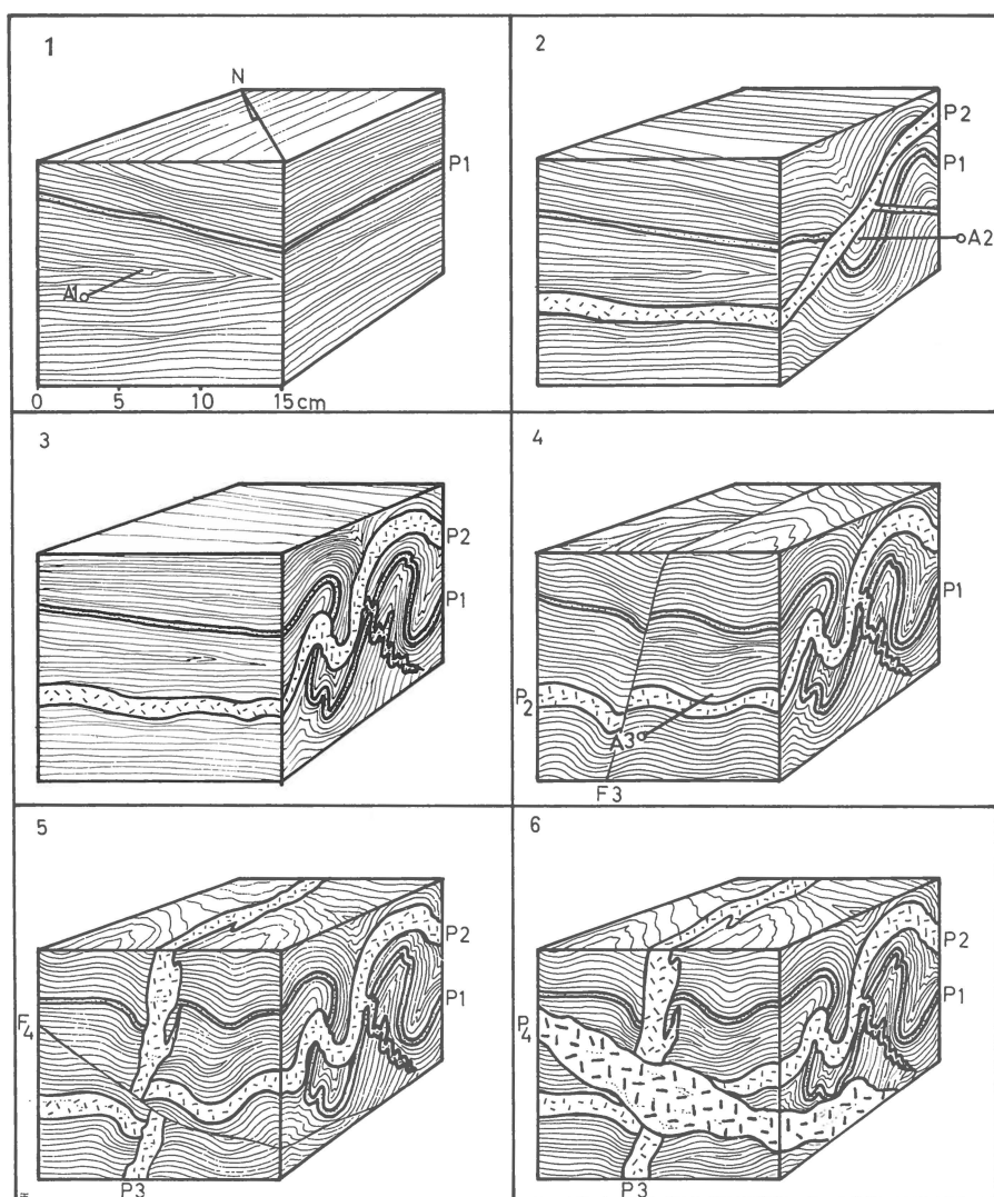
Fig. 23. Six theoretical stages during the Ketilidian deformations and pegmatitisation: 1) End of isoclinal folding I with axis A 1; emplacement of pegmatite P 1 along bedding or axial-plane cleavage. 2) Beginning of folding II with axis A 2; emplacement during this folding of pegmatite P 2 along slip planes parallel to the axis A 2. 3) End of folding II. 4) Beginning of folding III with axis A 3; formation of strain-slip cleavage plane F 3. 5) Continuation of folding III: emplacement of pegmatite P 3 along plane F 3, formation of fault F 4. 6) Formation of large pegmatite P 4 along plane F 4; end of folding III.
