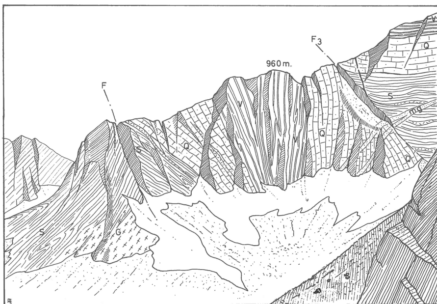
Fig. 5. View of the southern wall of the ridge coming down from Quvnerssuaq summit to lake 640 m. V = Volcanic rock; Q = Quartzites; S = Mica schists; G = Granite; F = Faults; mg = Microgranite.
