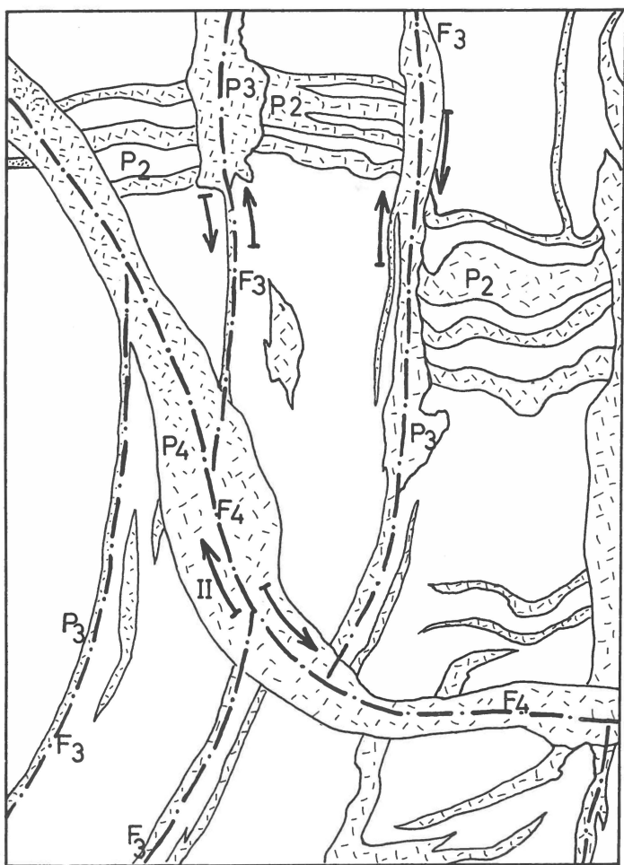
Fig. 22. Schematic interpretation of fig. 21, giving the probable directions of movement along the different fracture-planes (F 3, F 4) which gave birth to the pegmatites P 3 and P 4.
