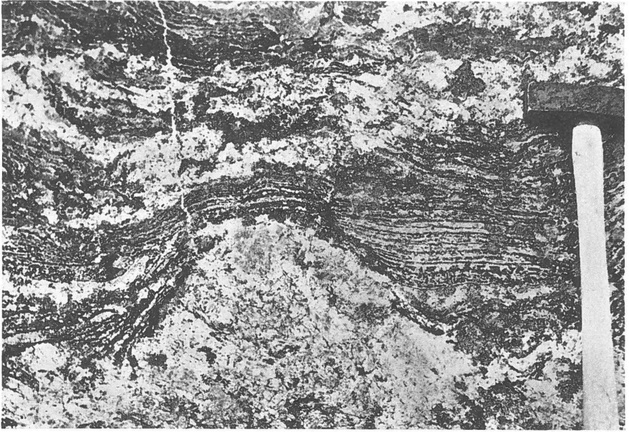
Fig. 18. Swell-structure on the border of a large fourth-generation pegmatite. It is obvious that the schist has been pushed aside plastically. Gneissic schist formation near Nanortalik harbour.
