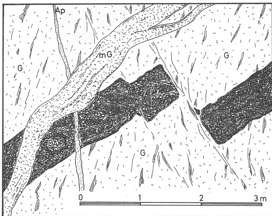
Fig. 35. Second generation metadolerite in granite A (G) near lake 560 m. The dyke contact transects inclusions. Dyke and granite are deformed by Sanerutian shearing and are cut by later microgranite (mG).
