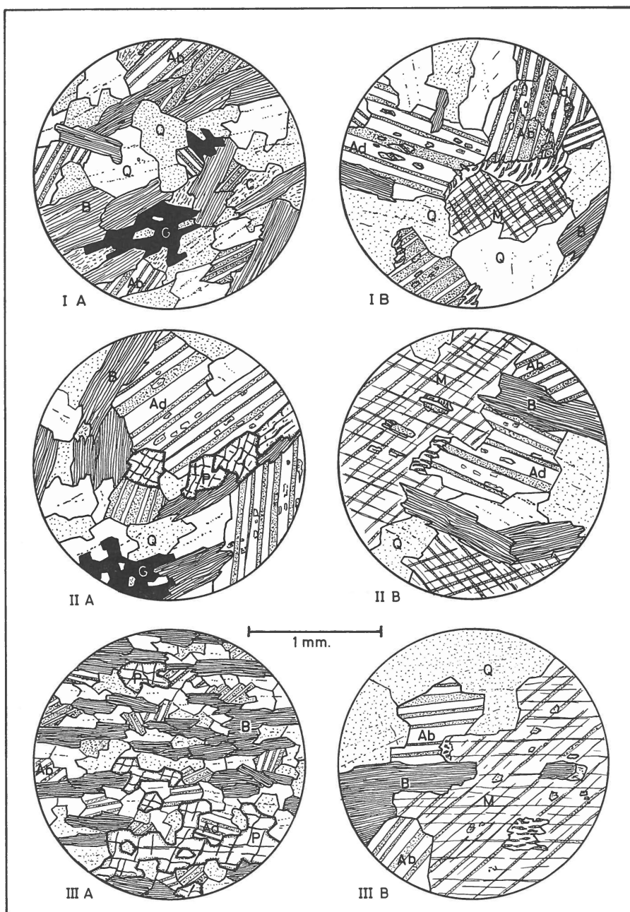
Fig. 30. Three stages of granitisation of garnet schists. The map on fig. 29 shows where the samples were taken. Q = quartz, M = microcline, Ab = albite-oligoclase, Ad = andesine, B = biotite, P = pyroxene, G = garnet, C = chlorite. For further explanations see text.
