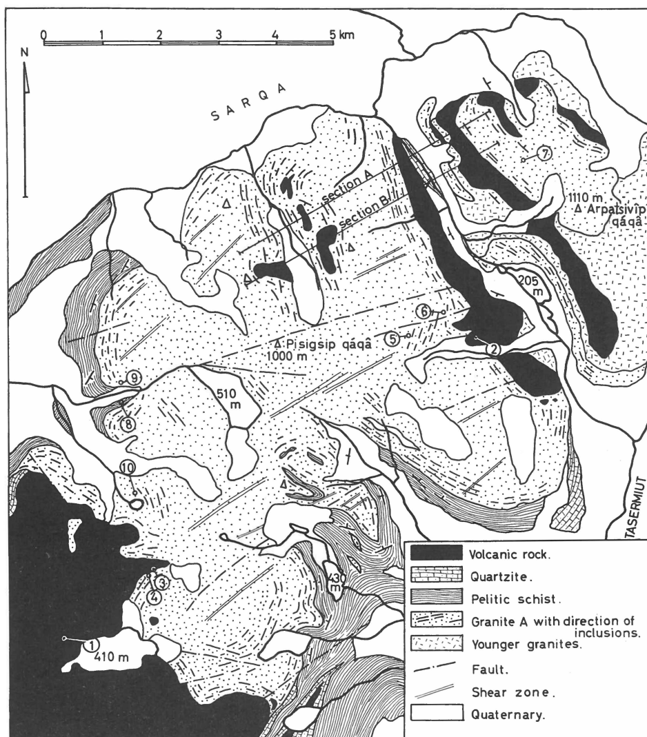
Fig. 28. Geological map of the central part of the Nanortalik peninsula, showing granite A and the directions of the foliation found in the inclusions. Nos. 1 to 10 correspond to samples taken for chemical analysis. Sections A and B correspond to those on fig. 26.
