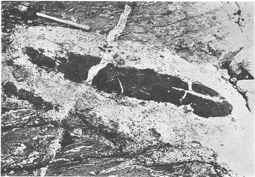
Fig. 34. Relicts of metadolerite enclosed in fine-grained microcline granite. Garnet schist formation near lake 430 m and near the contact with granite A.
