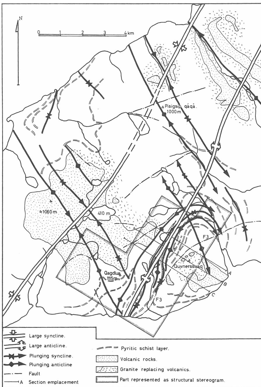
Fig. 3. Simplified structural map of the central part of the peninsula situated between Tasermiut and Sarqâ fjords.
