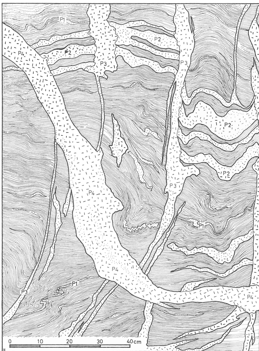
Fig. 21. Section normal to the third NNE fold-axes, showing the four generations of pegmatites. The P 3 veins follow the coarse strain-slip-cleavage planes formed during the third deformation period. Schist formation near lake 430 m. Drawn after a colour photograph.
