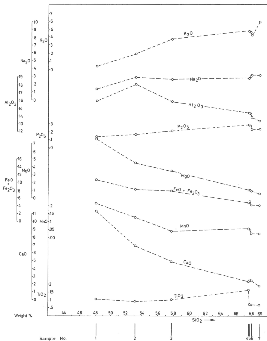
Fig. 33. A Harker variation diagram showing the differences in composition between pillow-lava and granite A in the contact zone between the two rocks. Nos. 1-3 represent lavas, nos. 4-7 were sampled in granites. The succession 1-7 corresponds to an increasing degree of granitisation.
