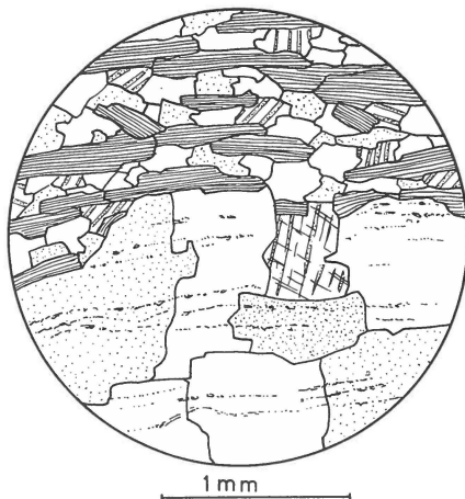
Fig. 15. Strings of inclusions in quartz in a small pegmatite vein near lake 430 m. The direction of the strings is clearly parallel to the elongation of the biotites in the schist. Slide No. 63631.
