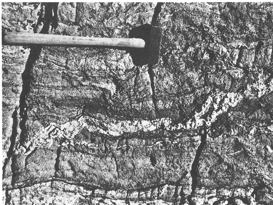
Fig. 13. Second-generation pegmatite in biotite schist near lake 430 m. The sub-concordant vein cuts and partially replaces the thin first-phase pegmatites.
