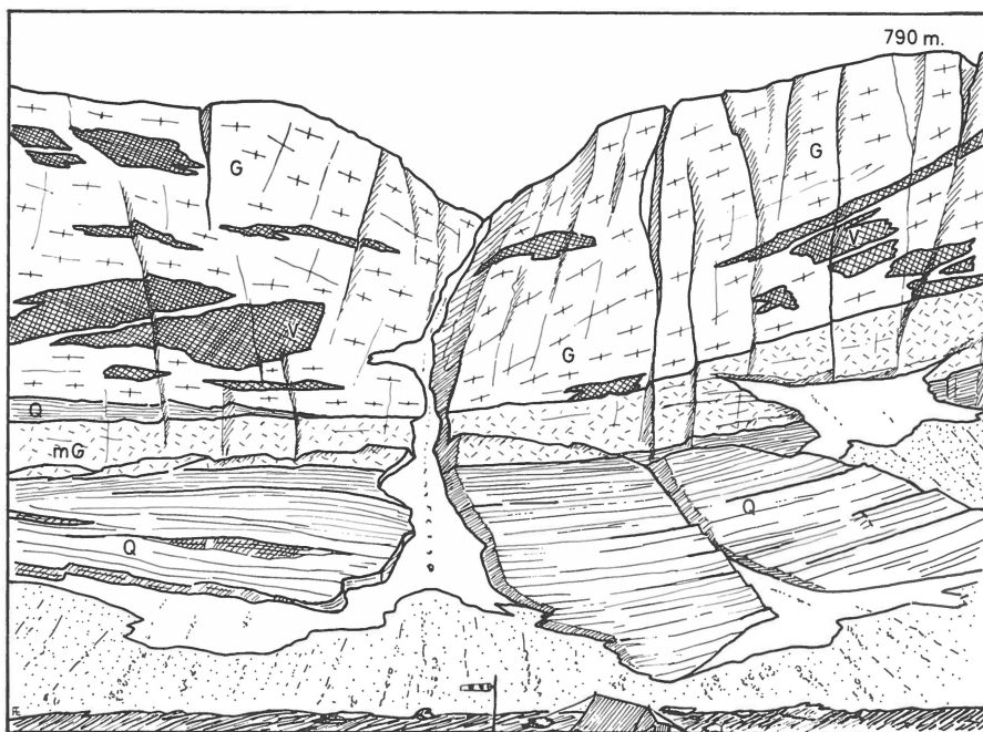
Fig. 31. NNW wall of Quvnerssuaq mountain. Granite A (G), containing large inclusions of volcanic rock (V), overlies conformably the quartzitic schists (Q). A later microgranite sheet (mG) follows more or less the contact.
