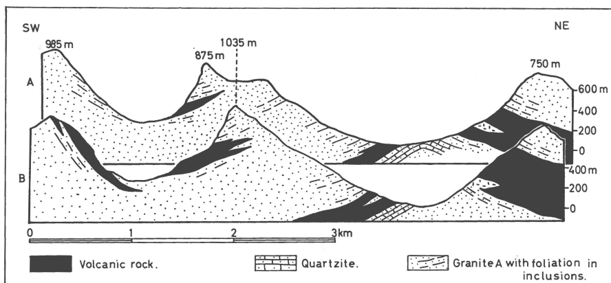
Fig. 26. Two schematic sections across granite A in the area N of Pisigisip-qâqâ mountain. The included relicts of volcanics and quartzites show the original structure before the granitisation. The trace of the sections is given on fig. 28.
