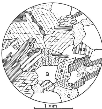
Fig. 9. Amphibolite. The amphibole (A) is corroded by quartz (Q) and albite (Ab). Biotite (B) is developed interstitially between two amphibole crystals. Slide No. 63647.
