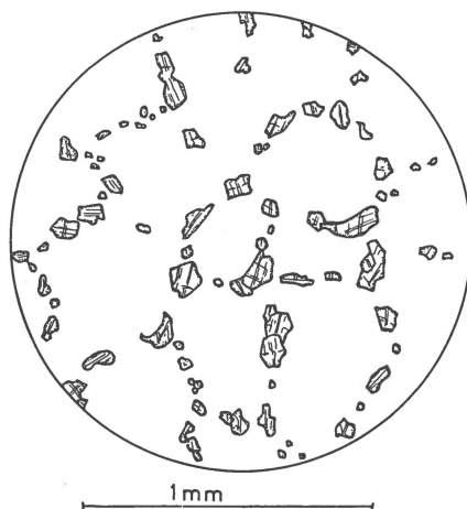
Fig. 10. Diopside crystal arrangement outlining the probable original borders of the clastic grains. The matrix is formed of finely crystallised quartz and feldspar. Quartzite near Tasermiut fjord. Slide No. 63607.
