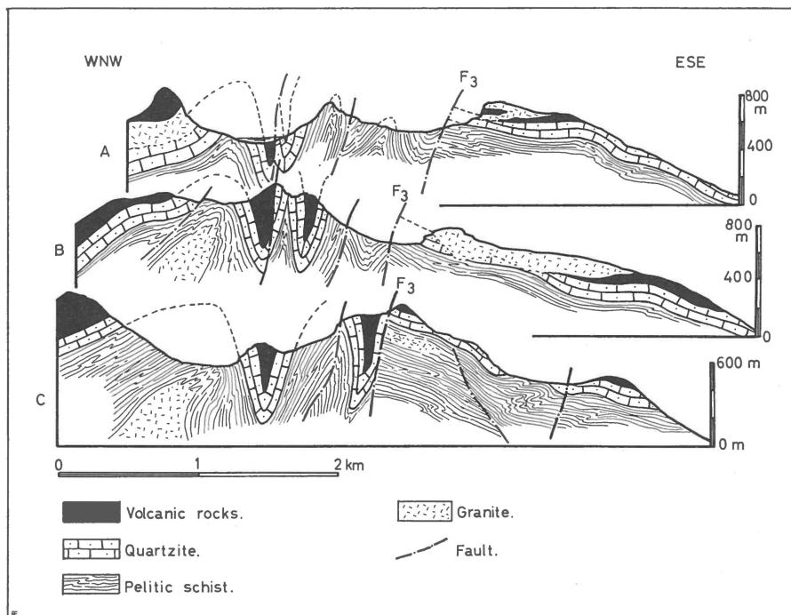
Fig. 4. Three hypothetical sections across the Quvnerssuaq mountain area. The exact position of the sections is represented on the map of fig. 3. The structures are a result of the first folding period.
