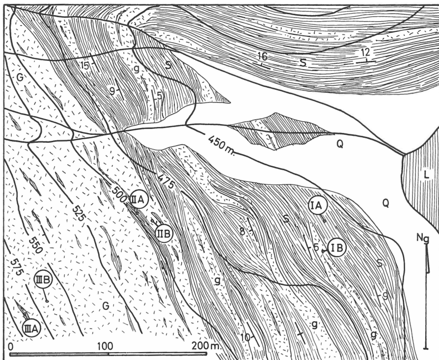
Fig. 29. Detailed geological map showing the contact zone between granite A (G) and garnet schist (S) W of lake 430 m. g = slightly granitised schist.
