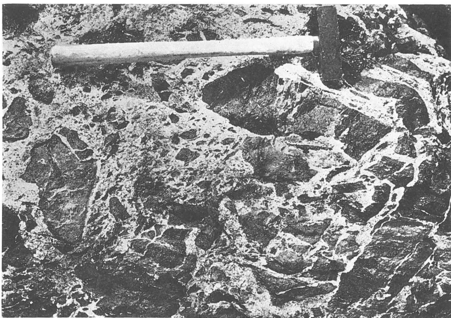
Fig. 32. Small-scale agmatite on the contact between granite A and volcanic rocks. Contact zone SW of lake 560 m (see geological map on plate 6).
