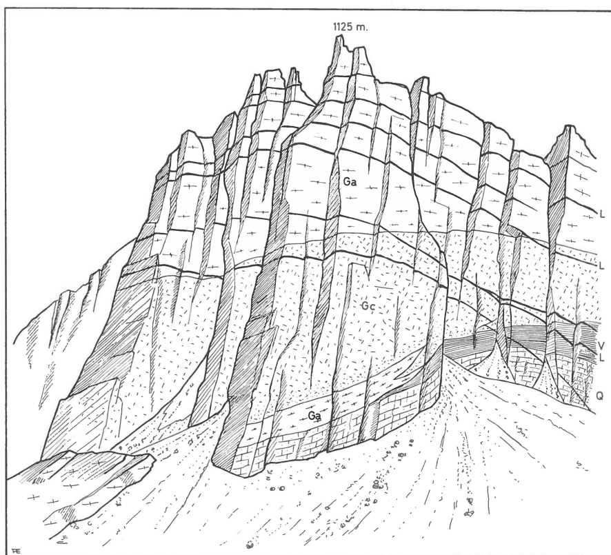
Fig. 39. View of the W wall of summit 1125 m in the Arpatsivîp-qâqâ mountain range, showing a huge sheet of granite C (Gc) lying between older granite A (Ga) and volcanic rocks (V). The whole structure is transected by numerous Gardar lamprophyre sheets (L).
