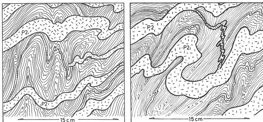
Fig. 19. Rock sections perpendicular to the second NW fold-axes. The P 2 pegmatites are clearly folded in the same direction as, but to a lesser degree than the schist layers. Schist formations around lake 430 m.
