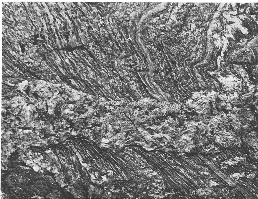
Fig. 17. Example of nondilation replacement pegmatite. Typical layers in the schist continue in the same plane on both sides of the vein. Third-generation pegmatite near lake 260 m. Width of the vein 20 cm.
