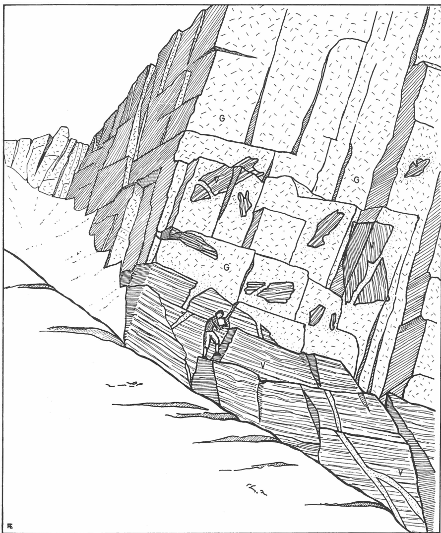
Fig. 44. North wall of mountain 1025 m in the Arpatsivip-qáqâ area, showing moved and rotated inclusions of volcanic rocks (V) in granite C (G) near the contact between granite and volcanics.
