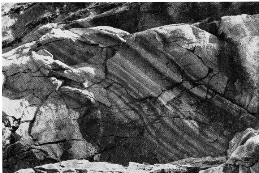
Fig. 12. Sharp conformable bands of alternating green and black lujavrites. South shore of Tunugdliarfik fjord.
