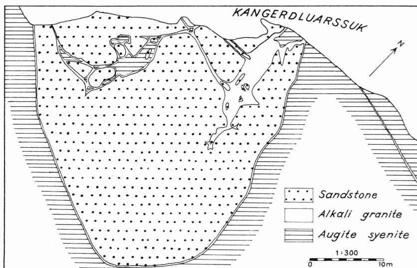
Fig. 7. Map of sandstone block in augite syenite with alkali granite formed as a reaction product.
