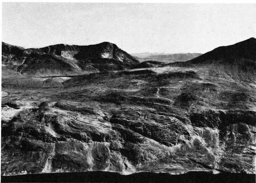
Fig. 25. Kakortokites viewed from Nunasarnaussaq.
