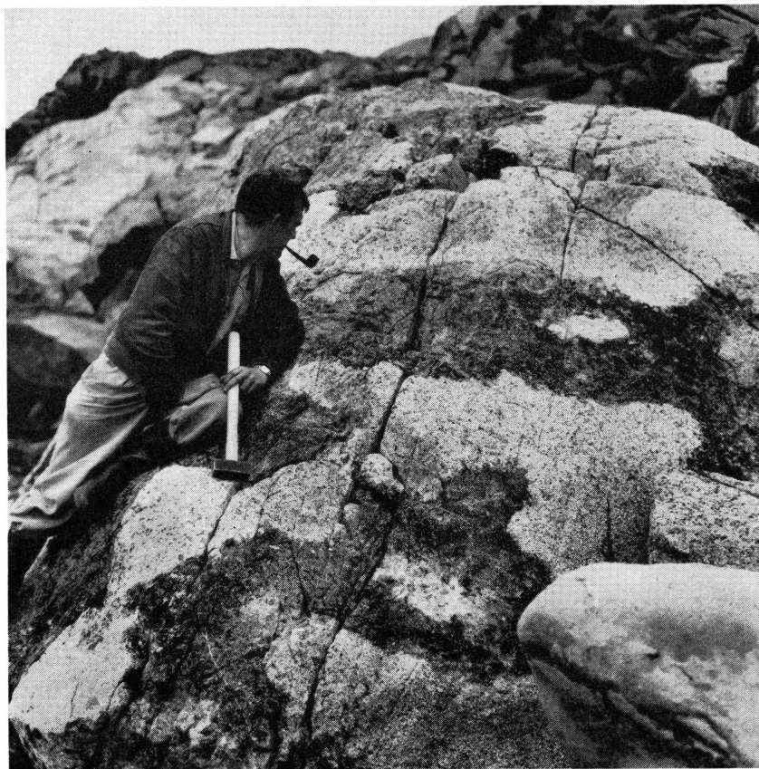
Fig. 21. Giant crystals 1–2 m long developed in naujaite. South coast of Nunasarnaq.
