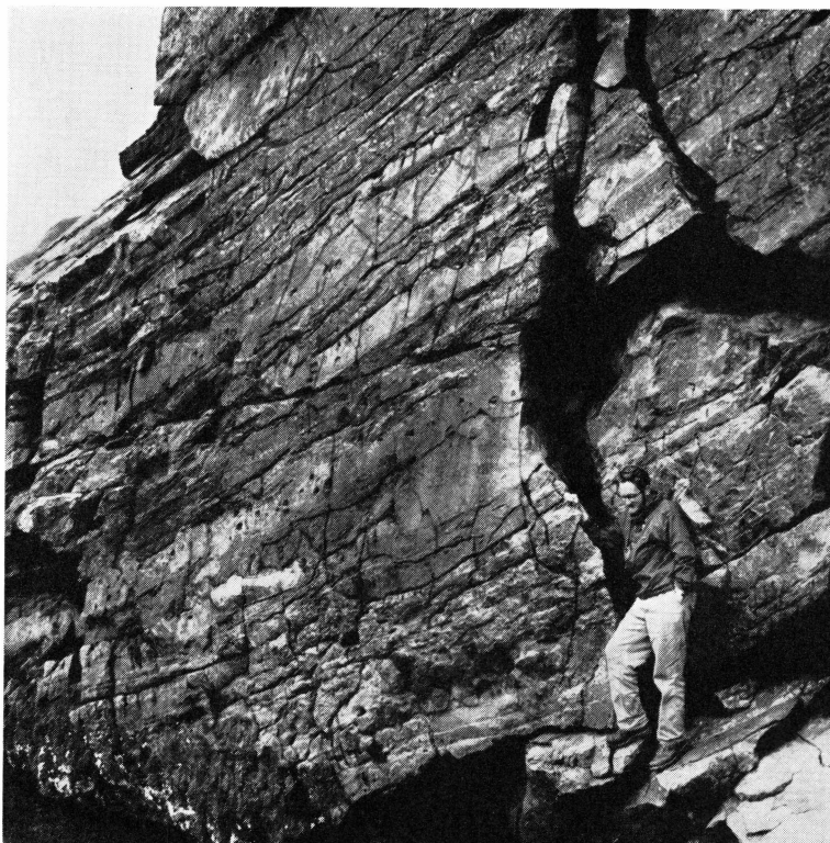
Fig. 35. Banding in black lujavrite produced by alternations of dark and light minerals, at Tugtup agtakôrfa.
