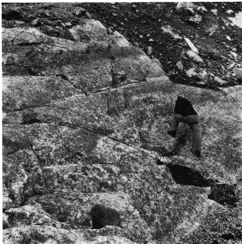
Fig. 23. Banding in naujaite. East of Igdlúnguaq.
