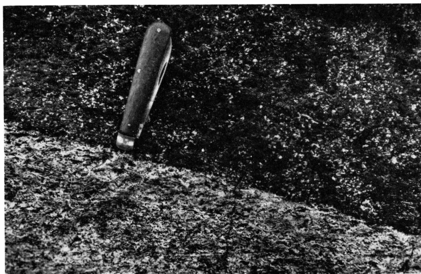
Fig. 29. Unusual razor-sharp contact between black and white kakortokite. Loc. Kringlerne plateau.
