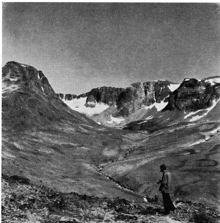
Fig. 2. Northern part of the Ilímaussaq Intrusion viewed from Kvanefjeld.
