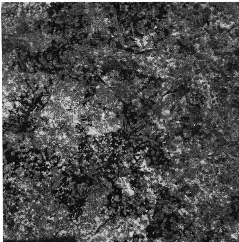
Fig. 20. Poikilitic texture of naujaite. Approx. scale 1:2.
