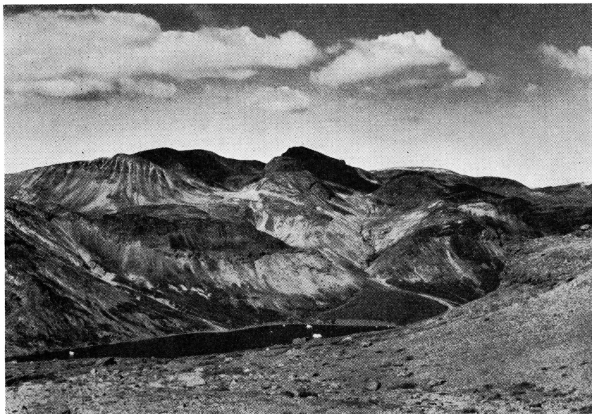
Fig. 3. General view of Ilímaussaq Intrusion north of Tunugdliarfik Fjord.
