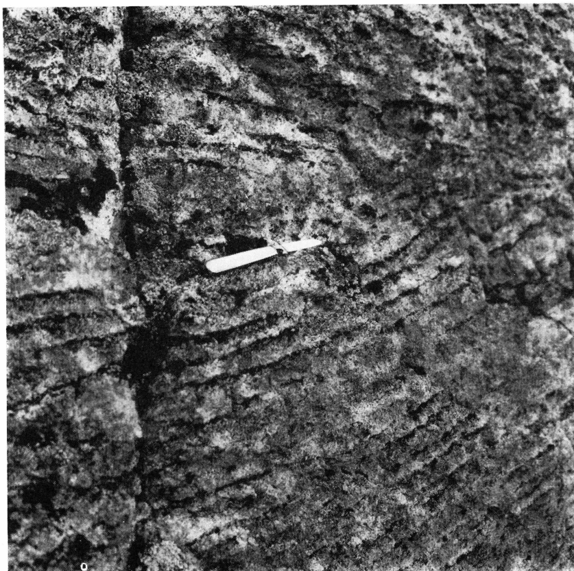
Fig. 18. Banding in quartz syenite sill with slight discordancy near the centre. 1 km northeast of Nunasarnaussaq.
