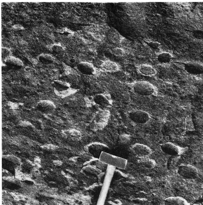
Fig. 38. Analcime nodules with acmite rims, in black lujavrite at Igdlúnguaq.
