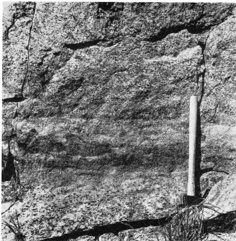
Fig. 37. Compositional and textural banding in nodular green lujavrite.
