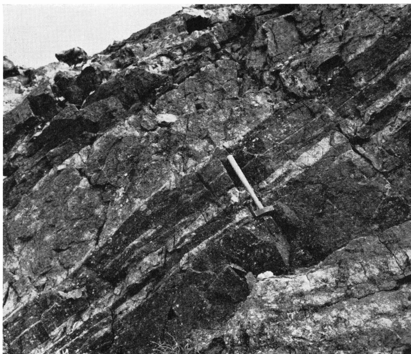
Fig. 34. Banding due to alternations of aegirine and arfvedsonite lujavrite.
