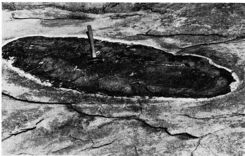
Fig. 13. Lens of "black lujavrite" or lujavritized basalt, in green lujavrite. West end of Nunasarnaq peninsula.
