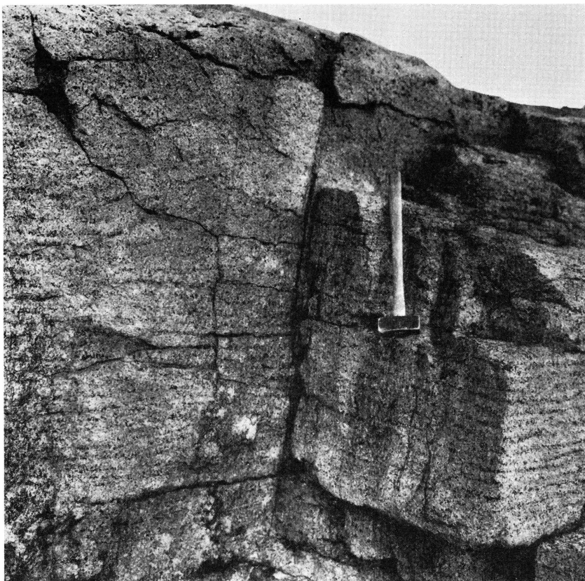
Fig. 19. Banding in pulaskite. 1 km north east of Nunasarnaussaq.
