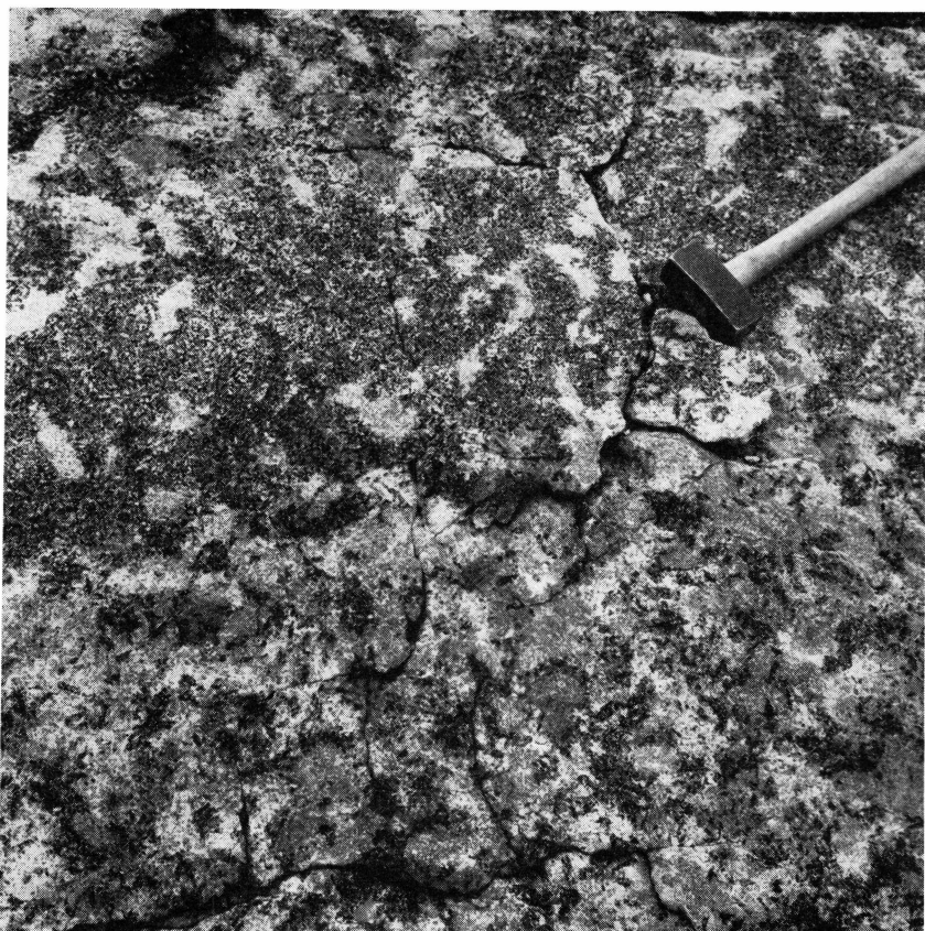
Fig. 24. Close-up of naujaite banding seen in fig. 23.
