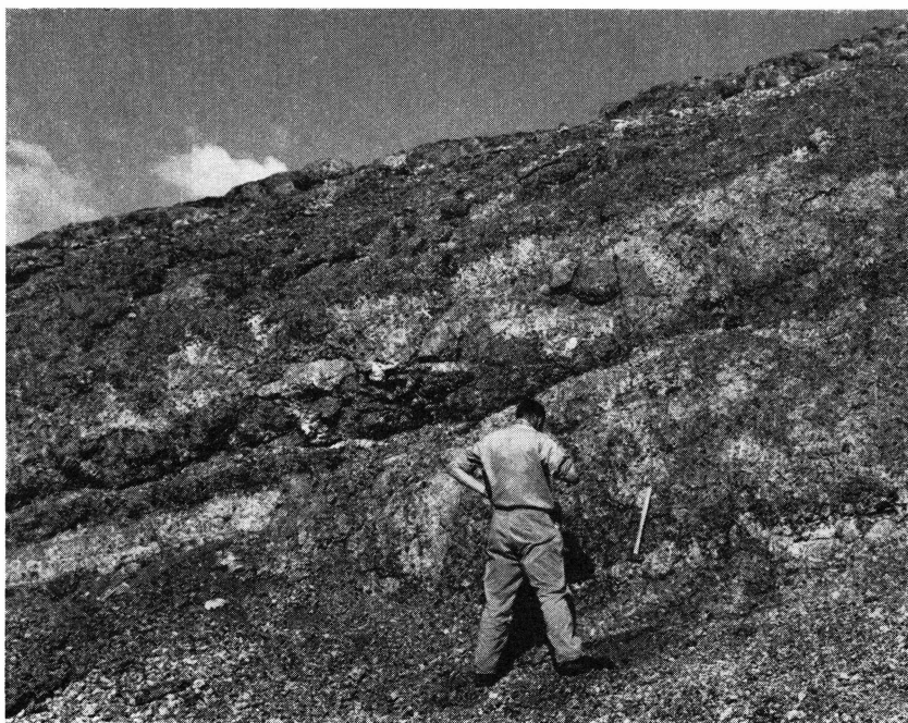
Fig. 17. Close up of banding seen in fig. 16.
