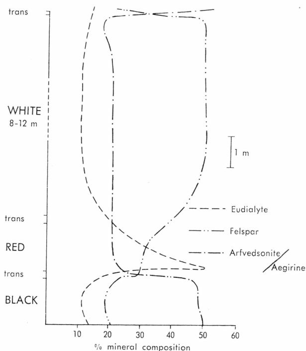
Mineral variation in layered kakortokites
