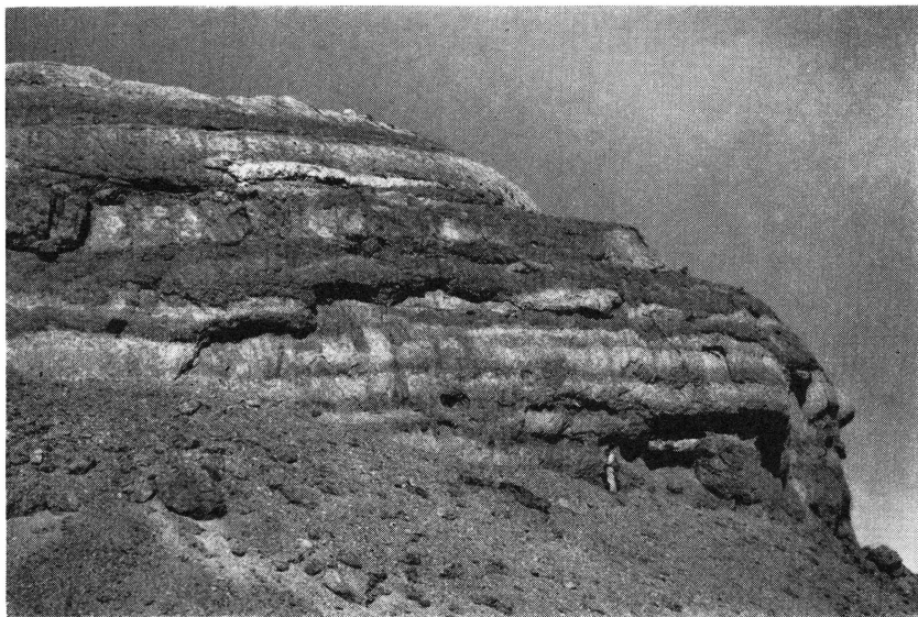
Fig. 16. Banding in heterogeneous syenite. 4 km north-east of Nunarsa- naussaq.
