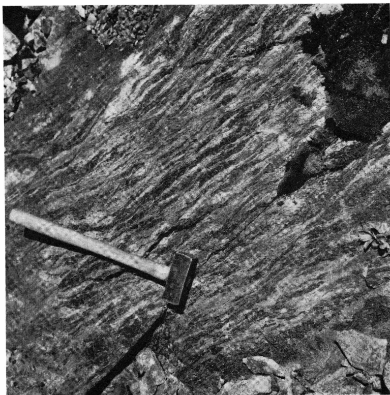
Fig. 22. Stretched naujaite. N.W. of Taseq lake.
