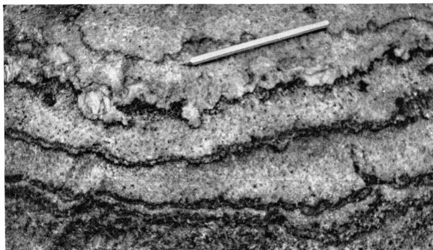
Fig. 4. Detail on an inclined surface of paired layers in the aplite. Note the slight irregularities in the paired layers with small pinch-and-swell structures (e.g. bottom left). The broad double layer in the upper half of the photograph contains many perthite crystals some of which have a zonal structure.
