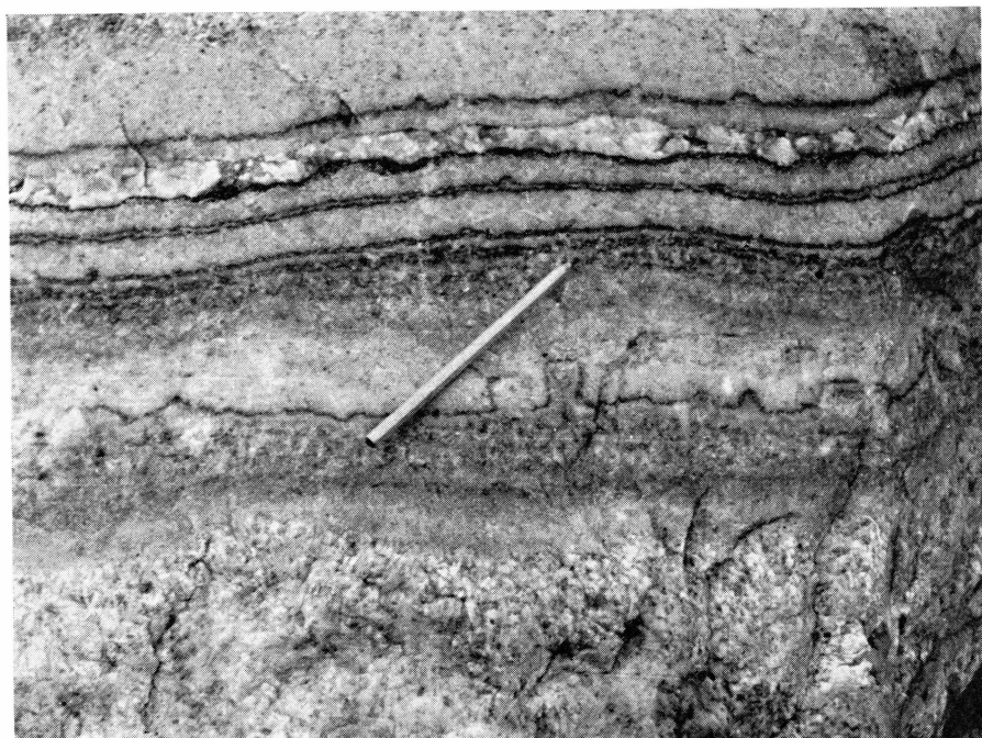
Fig. 3. Detail of layering within the aplite. Note the high proportion of paired garnet-bearing layers. A perthite-rich, coarse-grained layer is prominent at the top of the photograph. Eyed structures surrounding small perthite megacrysts are seen below the pencil. A concordant layer of quartz-felspar intergrowth is seen at the bottom of the photograph.
