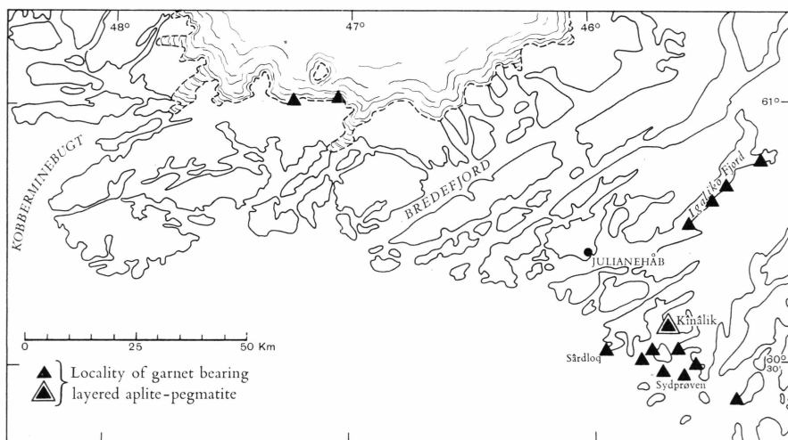
Fig. 1. Sketch map showing the distribution of garnet-bearing aplite-pegmatites in South Greenland.
