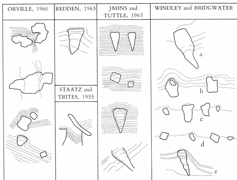
Fig. 6. Compilation diagram showing variable relations between potash feldspar megacrysts and surrounding layered aplite from different authors.
