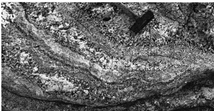
Fig. 9. Local development of aplite with garnet-rich layers near the upper surface of a sheet. Note that the garnet layering follows the irregularities of the pegmatite lenses.
