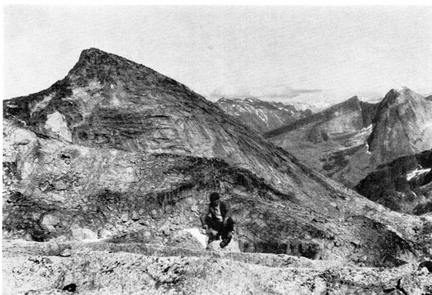
Fig. 7. Sheeting in the "new granite" SW of Kangerdlua bay, N Sermersôq. The curved planes of sheeting are convex towards the sky and parallel to the slope of the mountain (1030 m). Sheeting is present immediately below the niveau of the high-level erosion surface. Note the absence of other types of jointing in the sheeted granite.
