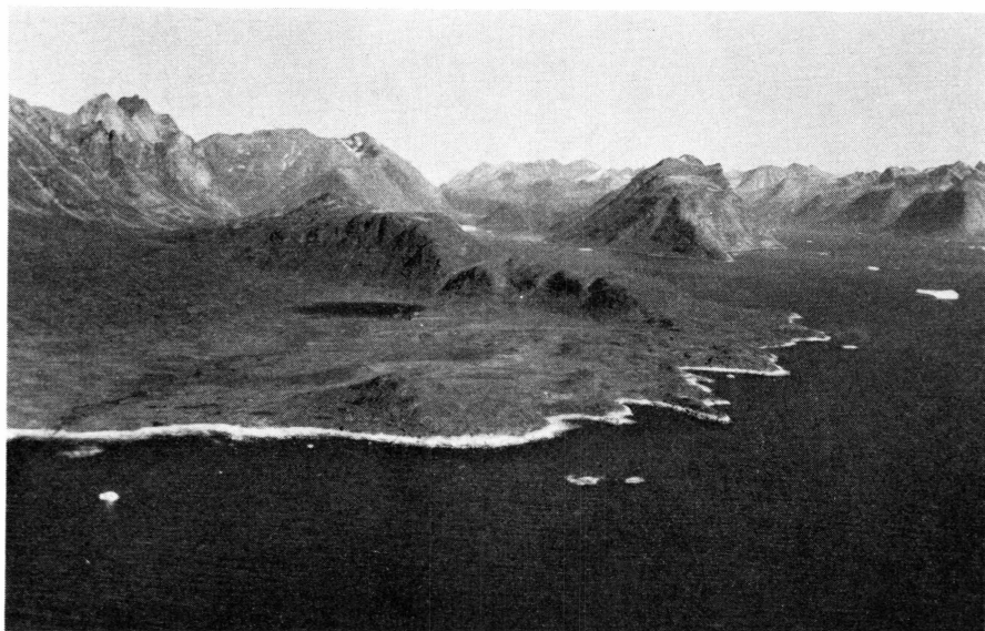
Fig. 6. The strandflat at Ikârissat viewed from the south. Away from the observer steep slopes separate the strandflat from small local flats belonging to the low- and intermediate-level erosion surfaces. In the background a summit level of over 1000 m indicates the high-level surface. (photo K. ELLITSGAARD-RASMUSSEN).
