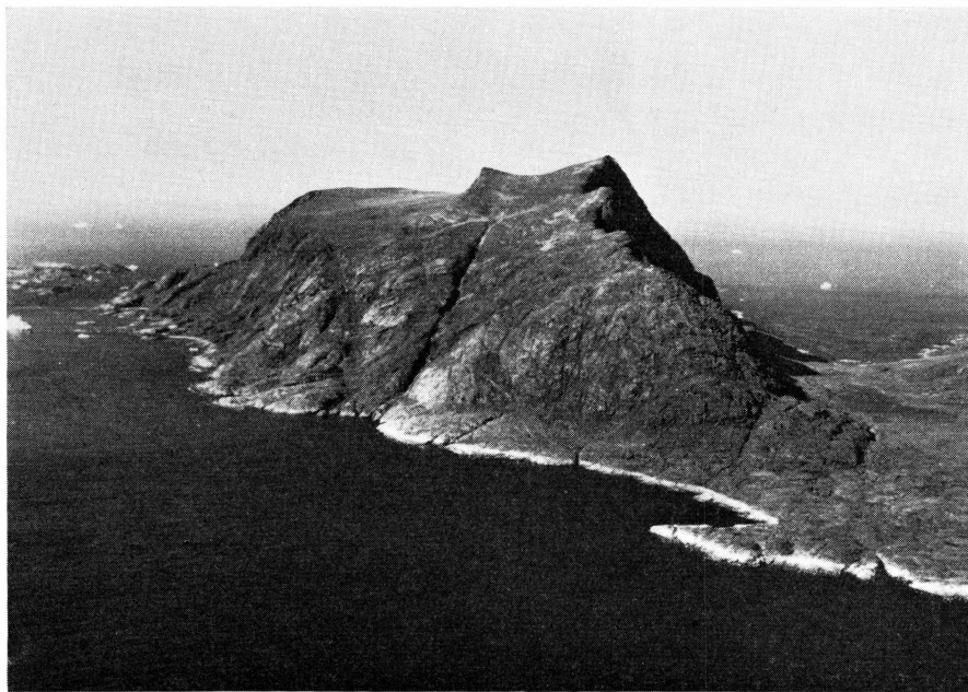
Fig. 5. The Itivdleq valley (right) and the peninsula south of this valley. The peninsula forms the southern part of Sermersôq and shows the intermediate-level erosion surface developed as a plateau with an average altitude near 600 m. In the foreground part of the strandflat is seen (photo K. ELLITSGAARD-RASMUSSEN).
