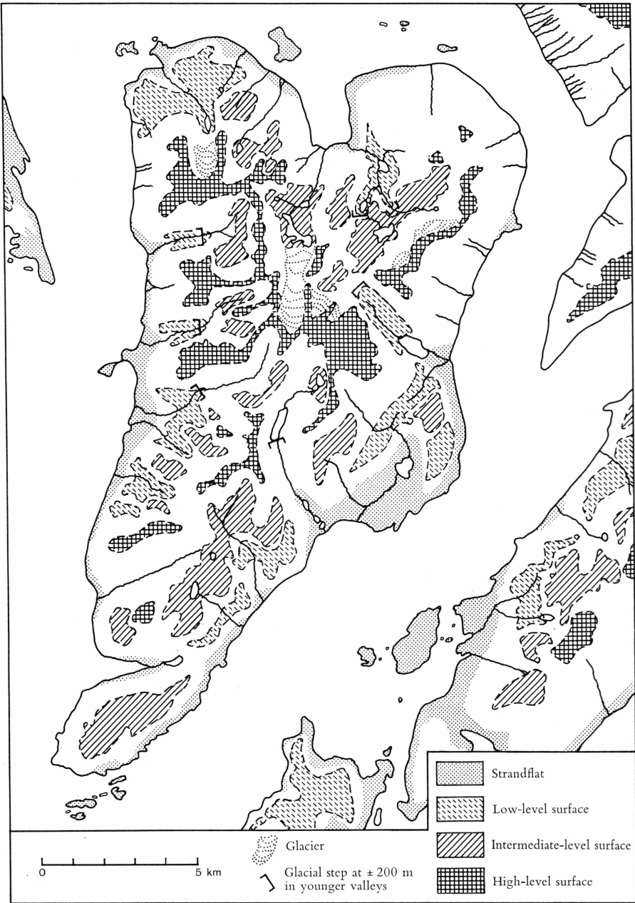
Fig. 2. The distribution of the four erosion surfaces on Sermersôq.
