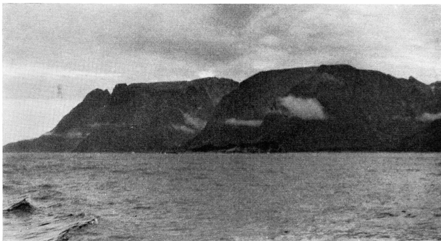
Fig. 3. The high-level erosion surface on northwestern Sermersôq viewed from the sea. The valley on the right-hand side of the picture is Kûgârssûk. In this region the high-level erosion surface forms high plateaus with an average altitude of about 1000 m.
