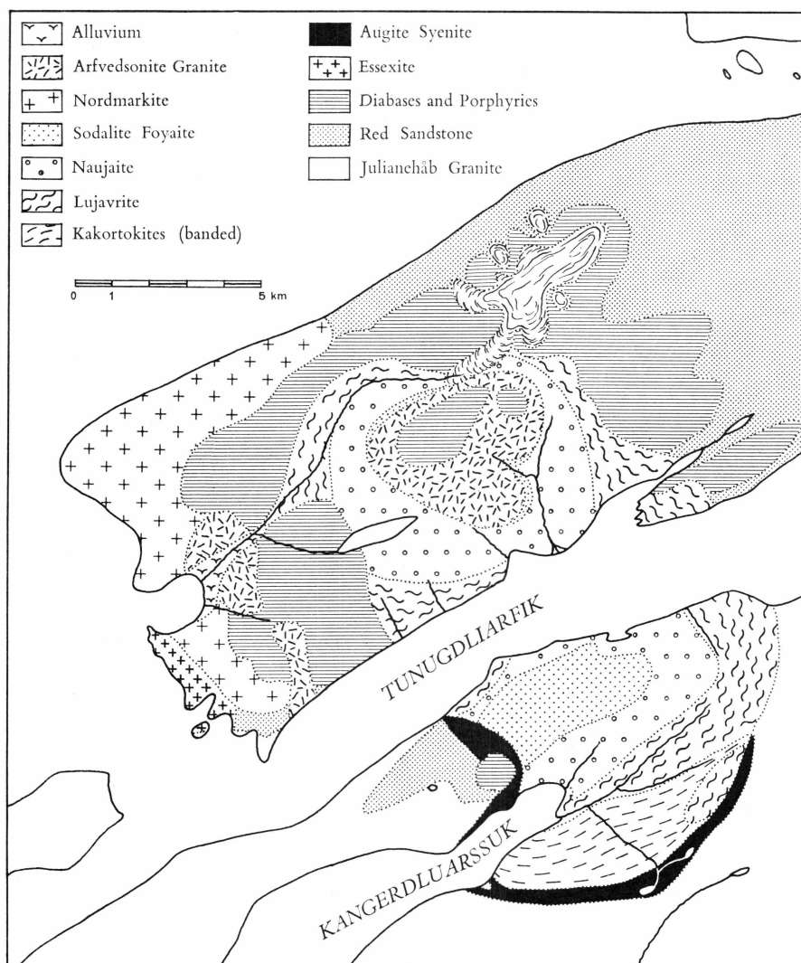
Fig. 7. USSING's geological map of Ilmaussaq modified with regard to contours and names of localities. The original map was printed in colour as plate 3 in USSING's memoir.
