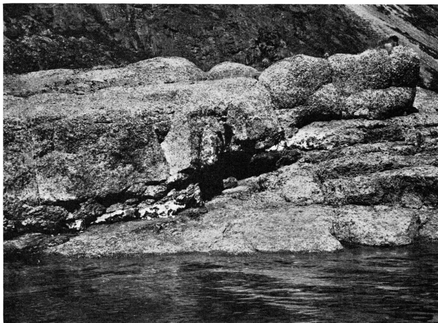
Fig. 3. Eudialyte-rich pegmatite in naujaite, Qeqertaussaq. The cave is a result of STEENSTRUP's excavations.
