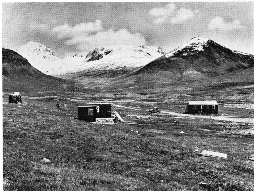
Fig. 9. Dyrnæs, the base of the present geological activity in Ilímaussaq. The snow-covered mountains in the background are Ilímaussaq (to the left) and Nákâlâq (centre). The dark mountain on the extreme left is Kvanefjeld. (BJARNE LETH NIELSEN phot.).
