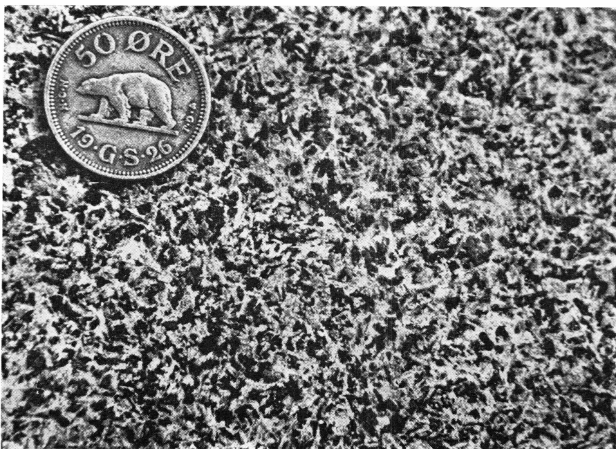
Fig. 13. Texture of metagabbro (3rd episode basic intrusion). The primary pyroxene has been partially replaced by hornblende but with the preservation of the ophitic texture. Diameter of the coin 2.2 cm. Photo: PREBEN CHRISTENSEN.
