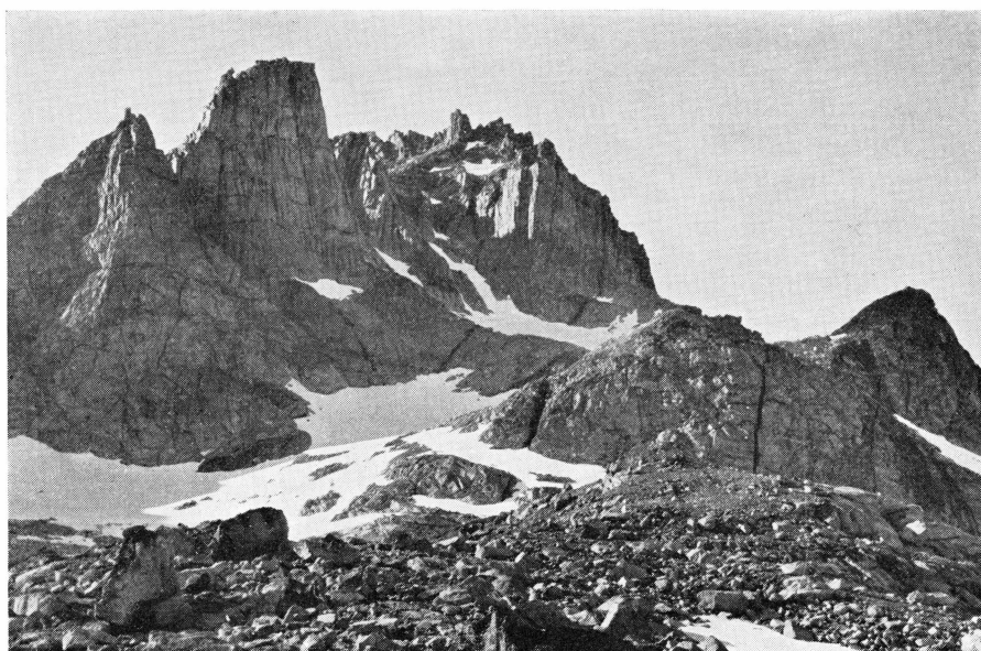
Fig. 11. Pyroxene-metadolerite dykes cutting sharply through Ketilidian granite and granitic gneiss. Younger basic sills are present in the higher parts of the mountains to the left.
