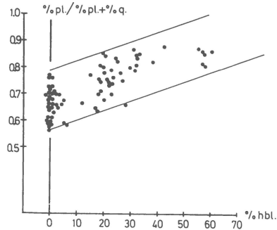
Fig. 15. Diagram showing the relation between the ratio % plagioclase/(% plagioclase + % quartz) and the hornblende content for the banded gneisses. The two parallel lines delimit the 95 % confidence belt within which most of the points fall. For further explanation see text. All the results from tables I a, I b and V have been plotted.
