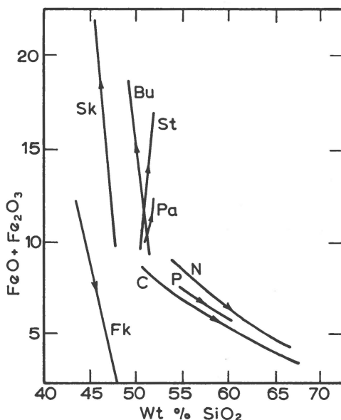
Fig. 37. A silica-total iron diagram showing liquid composition trends of various rock series including that of the Fiskenæsset complex (Fk). Curves for the layered intrusions: Bu = Bushveld; St = Stillwater; Sk = Skaergaard; Pa = Palisades diabase. Curves for calc-alkaline extrusive rock series: N = Nockolds' (1954) averages; P = Paricutin lavas; C = Cascades volcanic rocks (after OSBORN, 1969, fig. 6).
