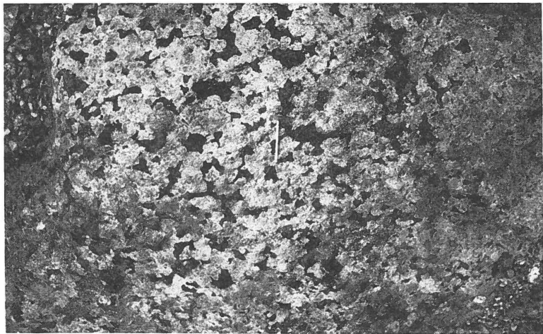
Fig. 22. Zone 5: Leuco-gabbro showing typical cumulate texture. Scale is given by the match. East of Fiskenæshumplen.
