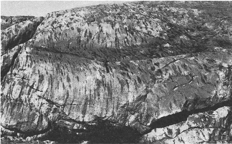
Fig. 24. Zone 6: Anorthosite containing elongate hornblendic schlieren. Hammer shaft is 40 cm long. Eastern Qeqertarssuatsiaq.
