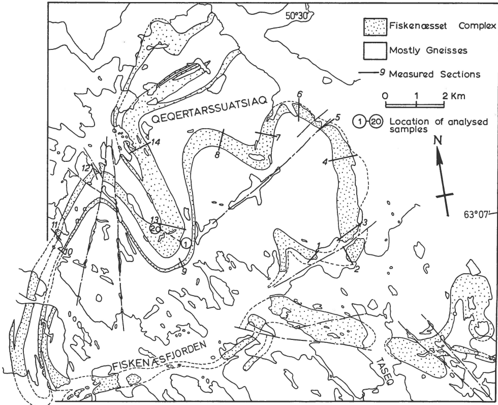
Fig. 2. Map of the Fiskenæsset complex in the Fiskenæs fjorden region showing the location of measured sections and analysed samples.
