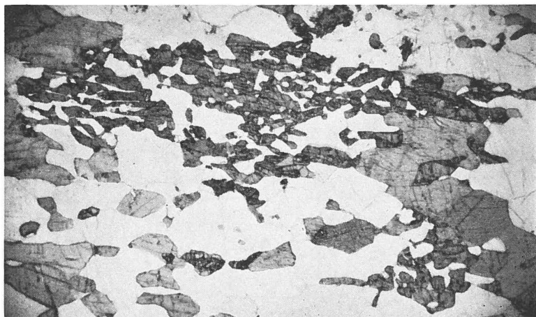
Fig. 6. Photomicrograph of spongy hypersthene-plagioclase intergrowth in hornblende norite of zone 3. The hypersthene granules are all in optical continuity. GGU 74497, plain light, \times 17 .
