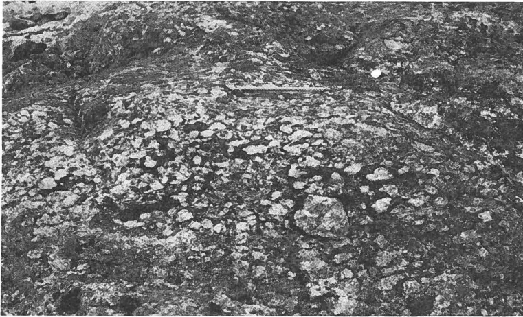
Fig. 27. Zone 7: Chromitite rich in plagioclase megacrysts. Scale is given by pencil. East of Taseq.
