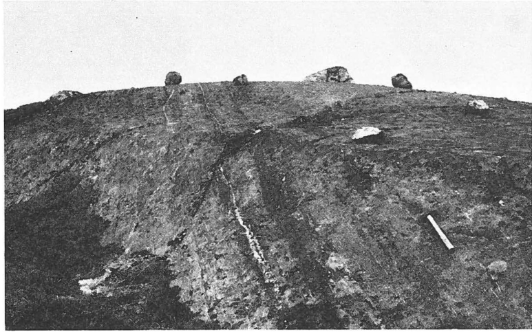
Fig. 15. Zone 1: General view of pyroxene amphibolite showing layering. Hammer shaft is 40 cm in length. Southern central Qeqertarssuatsiaq.
