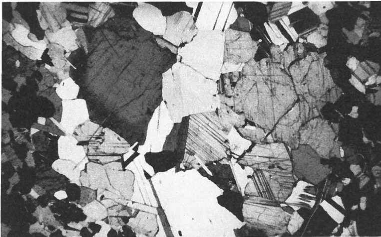
Fig. 13. Photomicrograph of zoned relict plagioclase within an augen in a hornblende-biotite chromitite matrix. Zone 7. GGU 86917, crossed nicols, \times 17 .
