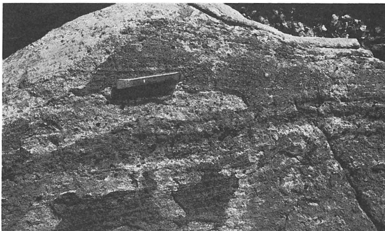
Fig. 30. Zone 8: Garnet anorthosite with garnets confined to certain layers. Southern central Qeqertarsuatsiaq.
