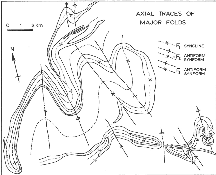
Fig. 40. Map giving the axial traces of the major folds in the Fiskenæs fjorden region.
