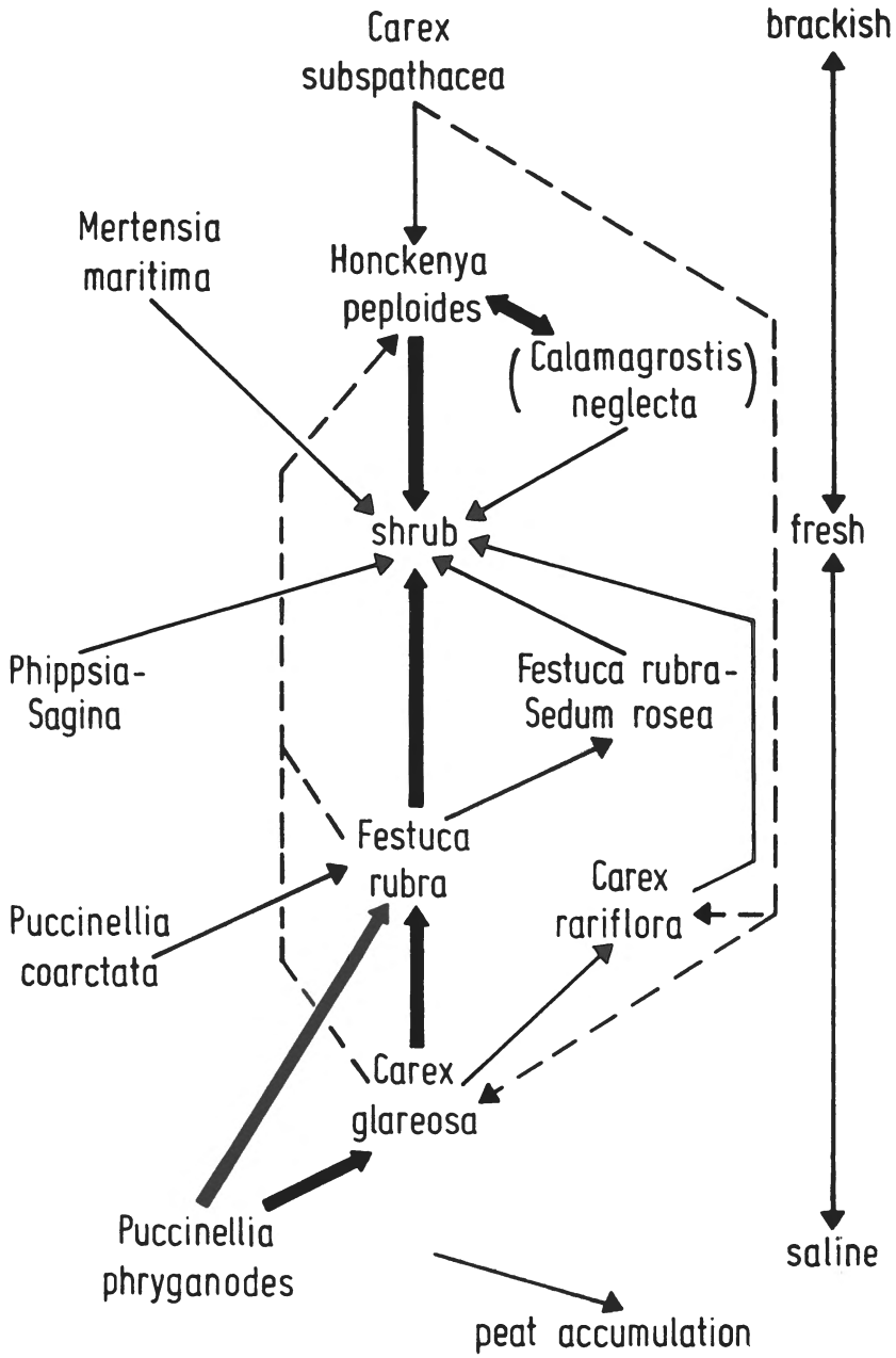
Fig. 13. Presumed succession of the littoral vegetation types in the Angmagssalik District; types indicated by the dominant taxa.
