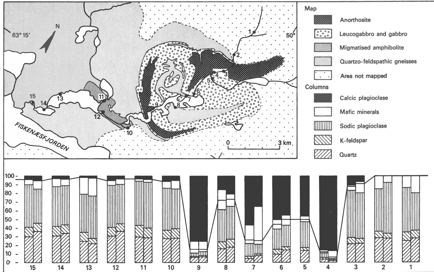
Fig. 10. Geological map of the Majorqap qáva area by JOHN MYERS (1973), and the localities where sand samples were collected. The columns show the mineralogical composition of the samples. There is a close agreement between the composition of the sands and the bedrock near the sample localities. The line between the columns divides anorthosite derived material (above) from gneiss/amphibolite derived material (below).
