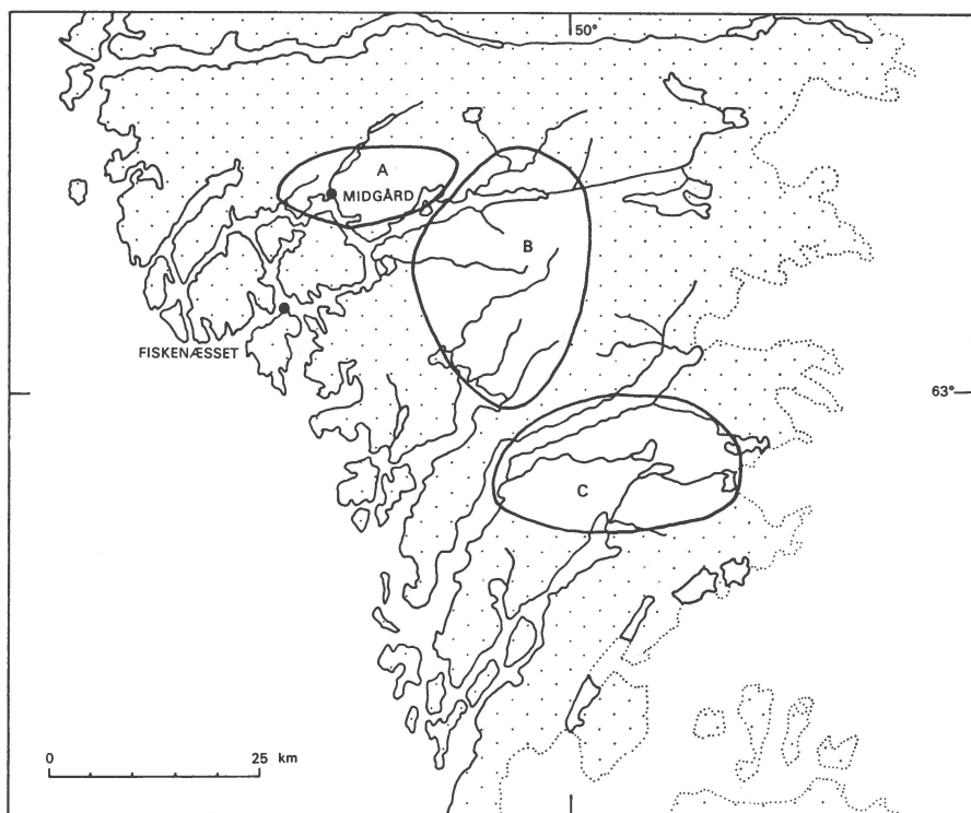
Fig. 5. Areas A, B and C from which mixtures of sands were analyzed. Sands from areas A, B and C differ in hypersthene contents, compare fig. 7.
