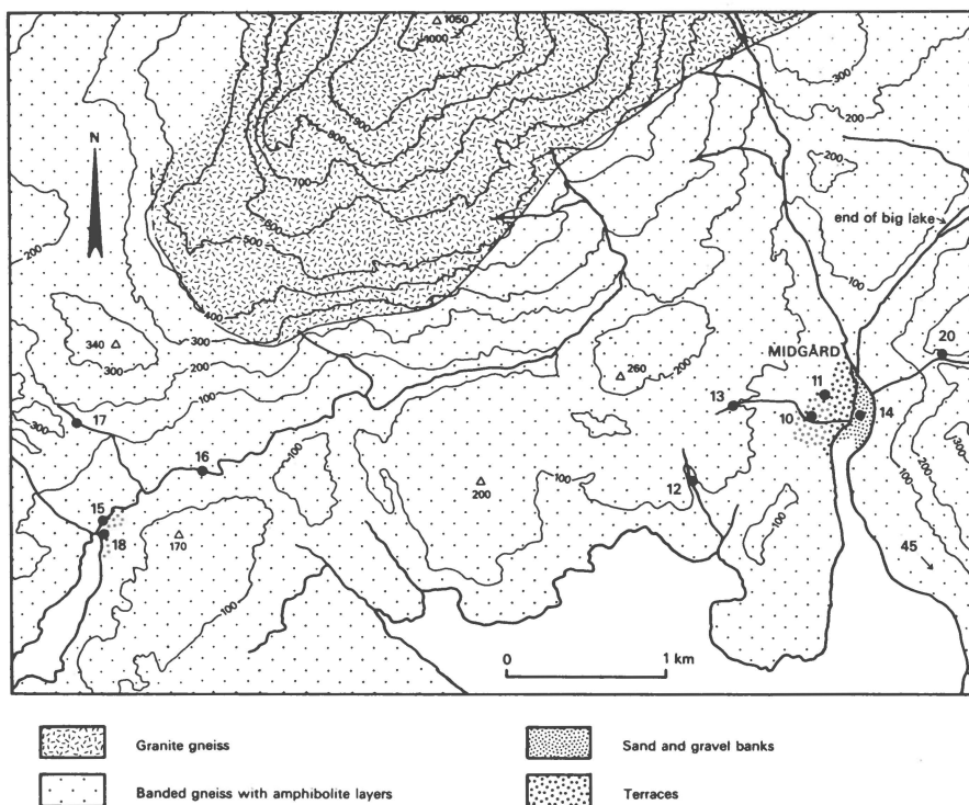
Fig. 9. Geological sketch map of the area around Midgård and the localities where sand samples were collected.
