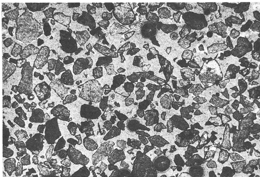
Fig. 1. Thin section of sand from the Fiskenæsset area. Note the angularity of the grains. The thin section is uncovered and the relief of the grains is therefore high. The largest grains are approximately 0.5 mm in size.
