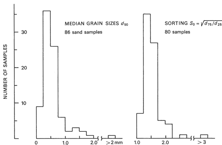
Fig. 6. Histogram of the median grain sizes d_{50} and the sorting coefficients S_0 = \sqrt{d_{75}/d_{25}} of the Fiskensæset sands.
