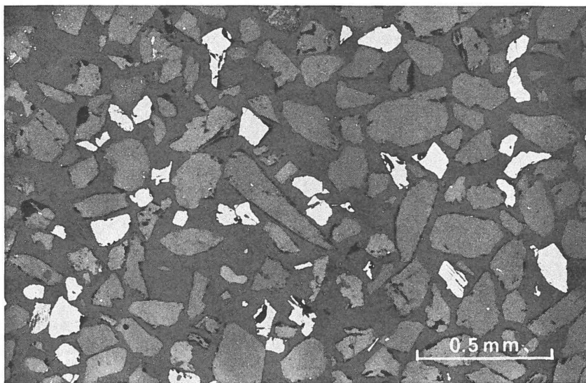
Fig. 8. Heavy fraction of sand from locality 10 under reflected light. Magnetite and ilmenite (white) and silicate minerals (grey) lying in 'Araldite'.
