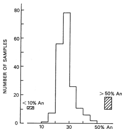
Fig. 4. Histogram of the An contents of 197 plagioclase grains from the Fiskensæset sands. The composition of the very calcic plagioclase from the anorthositic rocks is not shown in the diagram.
