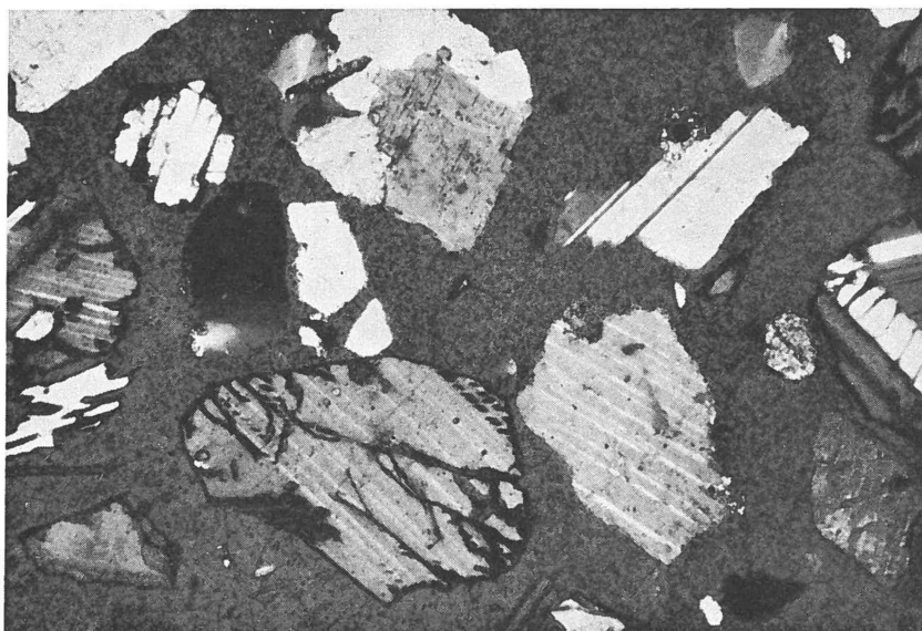
Fig. 2. Calcic (anorthosite-) plagioclase and sodic plagioclase with some quartz. The very calcic plagioclase has a high relief and is strongly etched by the HF vapours. The largest grain is 1.5 mm in size. Crossed polars.
