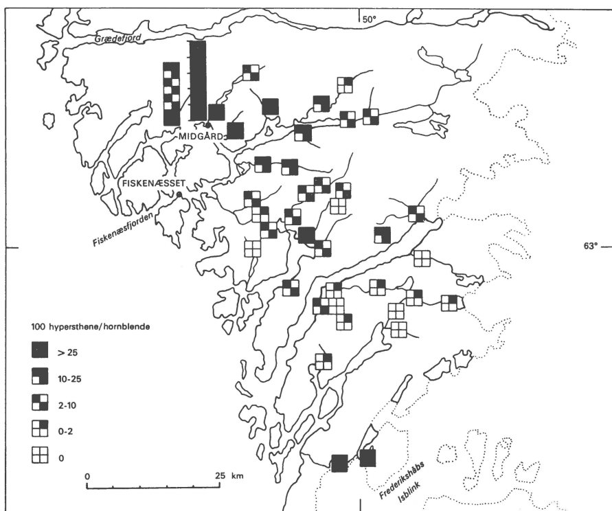
Fig. 7. Distribution of hypersthene in the sands from the Fiskenæsset area, expressed as 100 hypersthene/hornblende. The amounts of hypersthene and hornblende are given in KALSBECK, GHISLER & THOMSEN (1973).
