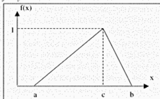
Figur 2. Membership funktion for triangulært fuzzy tal .
