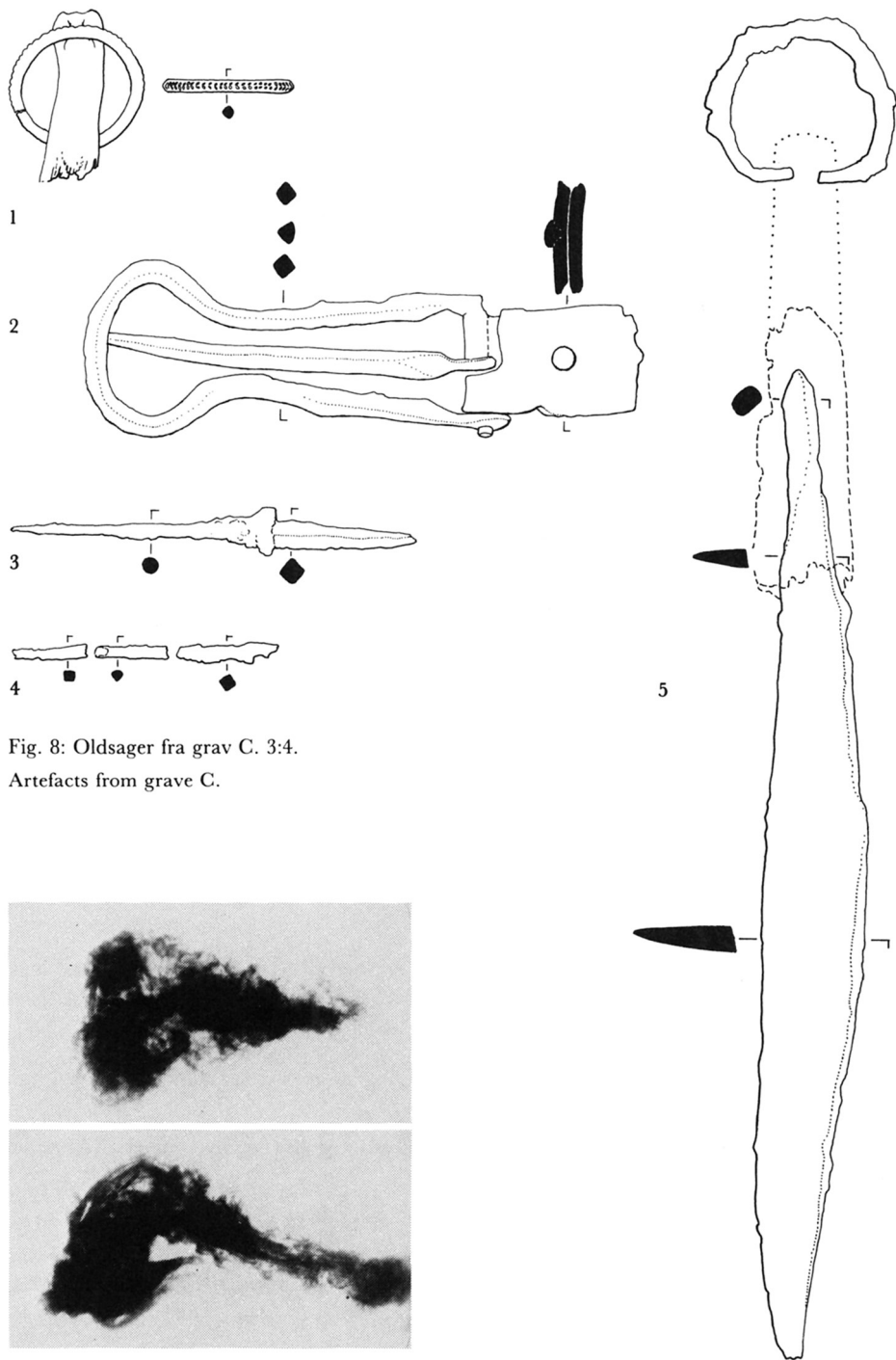
Fig. 9: Røntgenfoto af jernfibel fra grav C. X-ray photograph of iron fibula from grave C.
