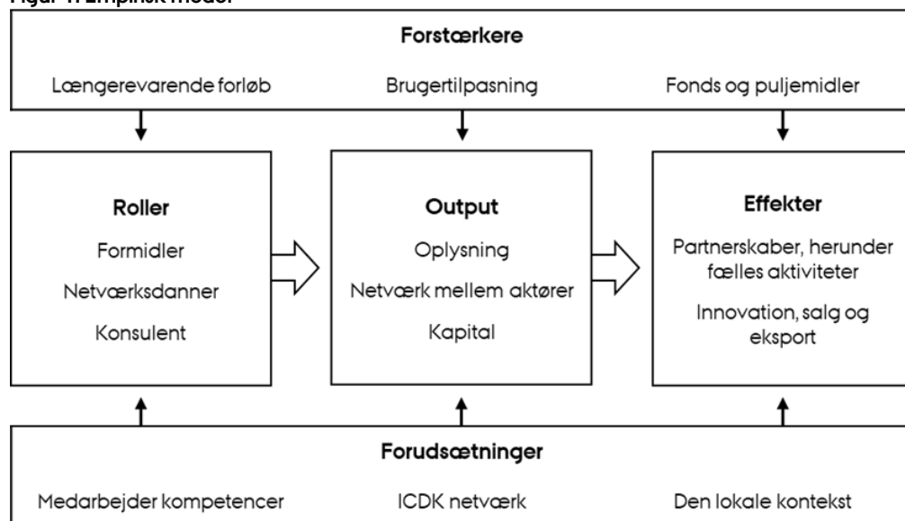
Figur 1. Empirisk model
