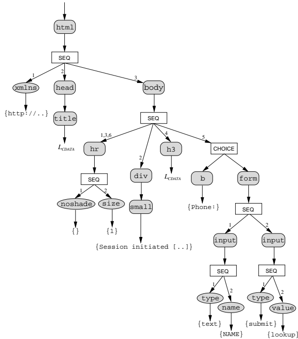
Fig. 2. Summary graph for the example program. (We depict element nodes as rounded boxes, attribute nodes as ellipses, and sequence and choice nodes as SEQ and CHOICE boxes, respectively. Edges out of sequence nodes are ordered according to the indices.)
