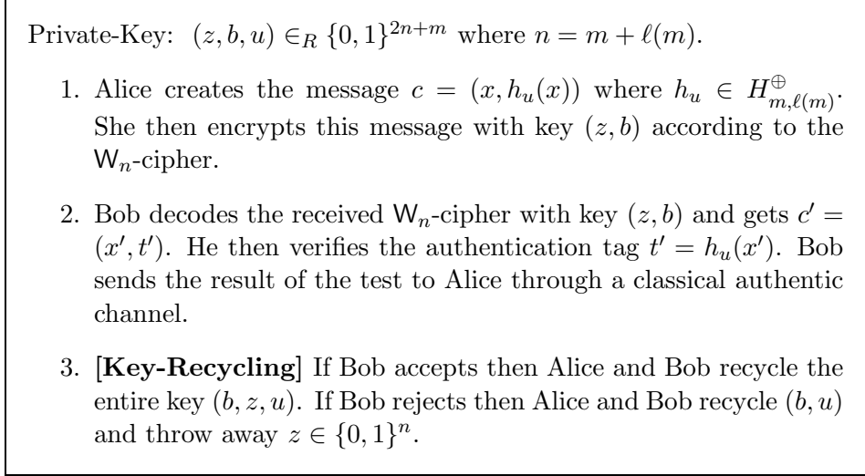
Figure 1: The W_nC_m .
