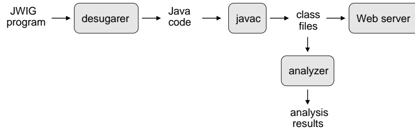
Fig. 6. The Jwig program translation process in our current implementation. The Jwig program is desugared into Java code which is compiled to class files. These class files are used both in the Web server and to perform the program analyses.
