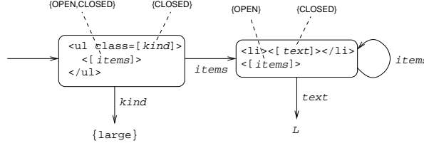
Fig. 12. A summary graph whose language is a set of XML documents, each containing a ul list with zero or more text items and a class attribute. The node on the left is a root, the dashed lines show the gap presence for each gap, and L denotes some set of strings.
