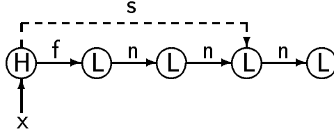
Figure 2: A list structure
