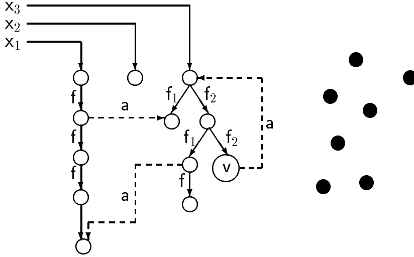
Figure 1: A rooted graph.
