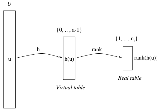
Figure 3: Overview of the dictionary for S_1
