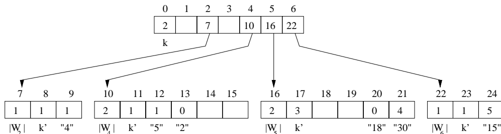
Figure 2: FKS scheme with quotienting
