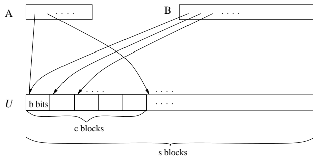
Figure 1: Splitting of U and structure of A and B tables
