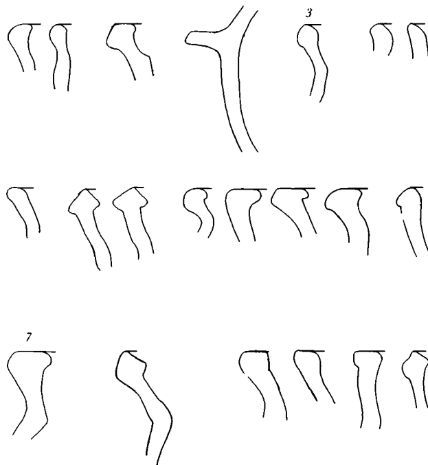
Fig. 8. Gruppe A2, randprofiler, ASR 152 × 1, × 2, × 3, × 4, × 5, × 6, × 7, × 10, × 11. Tegning: Jan Sloth-Carlson. 1:2.
